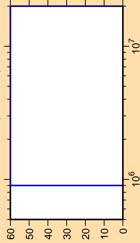
\Delta\sigma/\sigma vs. E for ^{161}\text{Ta}(n,\text{ncont.})
