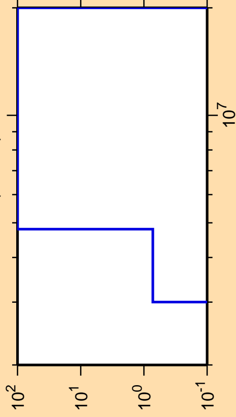
\Delta\sigma/\sigma vs. E for ^{161}\text{Ta} (mt 45)
