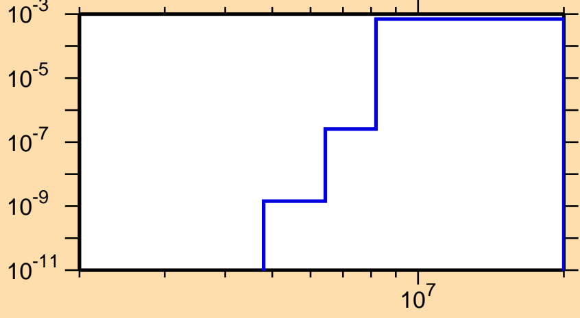
\sigma vs. E for ^{161}\text{Ta} (mt 45)
