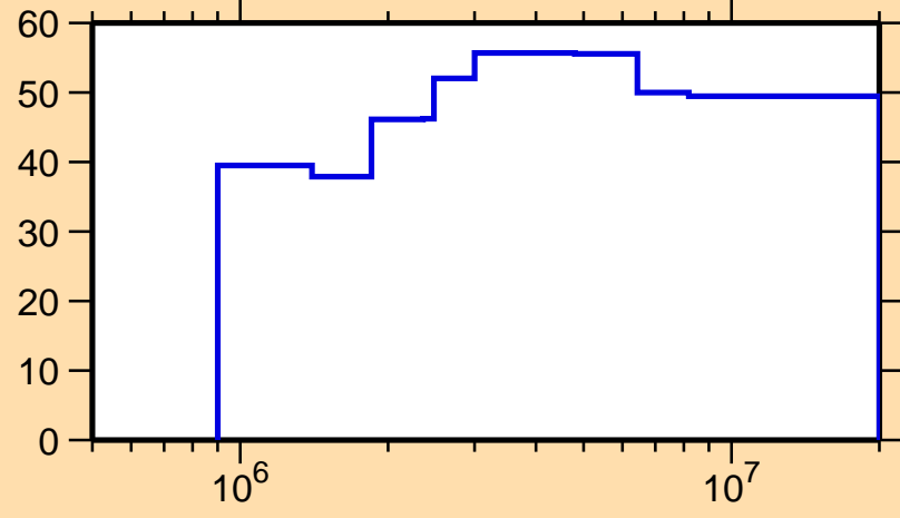
\Delta\sigma/\sigma vs. E for ^{161}\text{Ta}(n,n_1)
