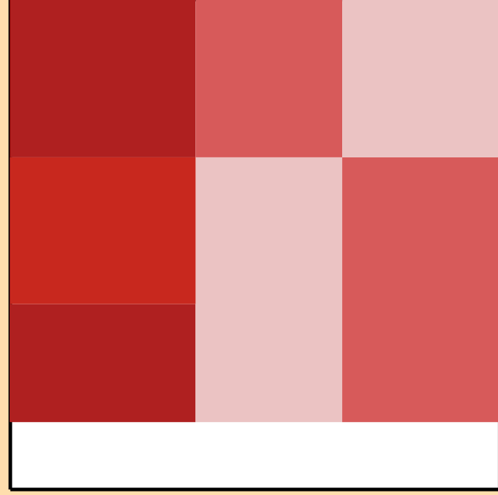
\Delta\sigma/\sigma vs. E for ^{161}\text{Ta}(n,\text{el.})
