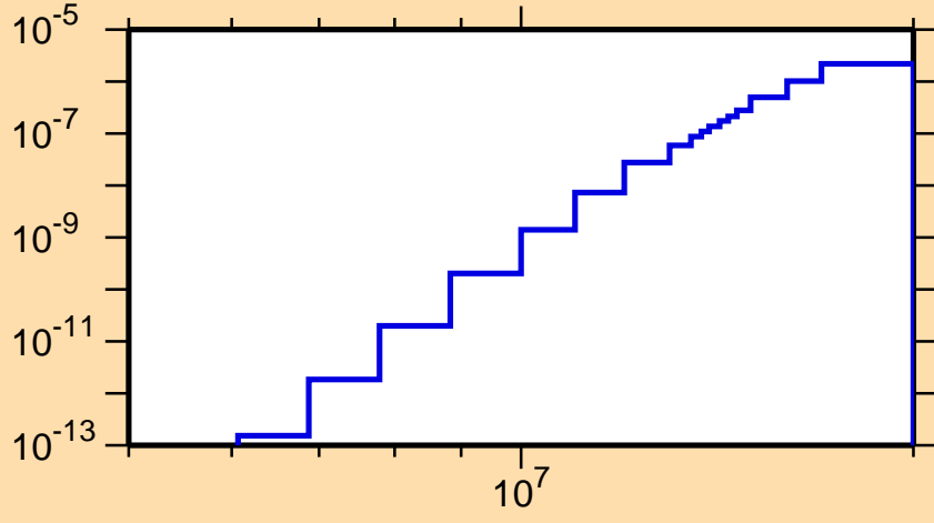
\sigma vs. E for ^{163}\text{Ta}(\text{mt117})
