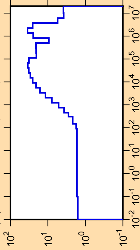
\Delta\mu/\mu vs. E for ^{163}\text{Ta}(\text{mt251})
