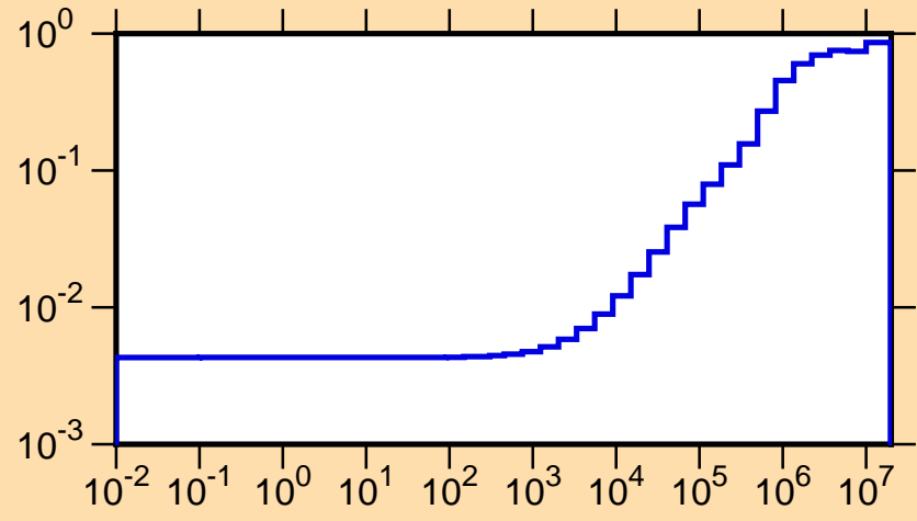
\mu vs. E for ^{163}\text{Ta}(\text{mt251})
