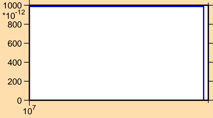
\sigma vs. E for ^{163}\text{Ta}(n,\text{pt})
