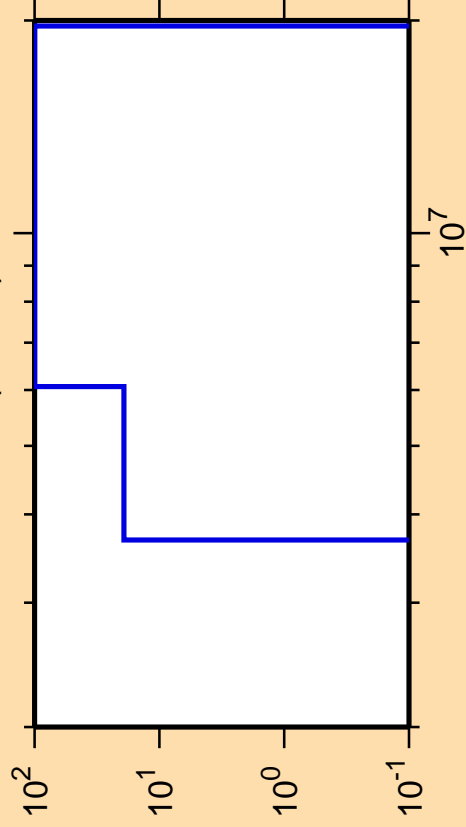
\Delta\sigma/\sigma vs. E for ^{163}\text{Ta} (mt 45)
