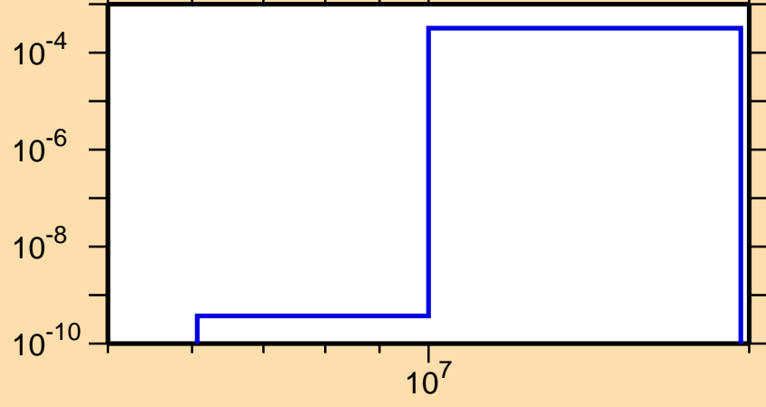
\sigma vs. E for ^{163}\text{Ta}(n,t)
