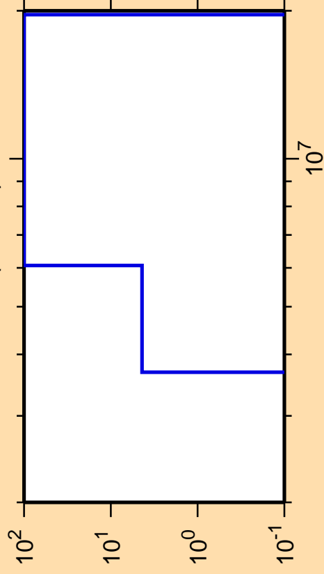
\Delta\sigma/\sigma vs. E for ^{163}\text{Ta}(n,\text{He}3)
