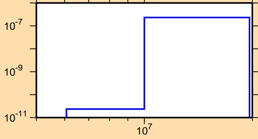
\sigma vs. E for ^{163}\text{Ta}(\text{mt117})
