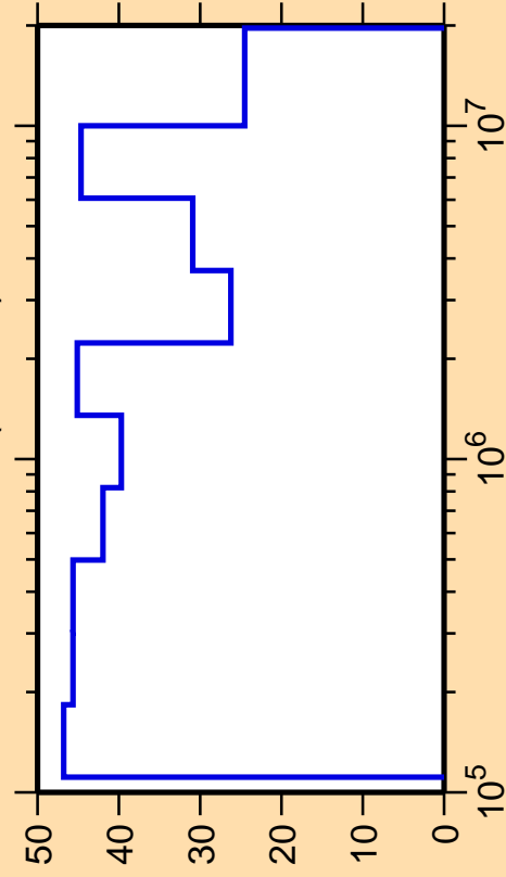
\Delta\sigma/\sigma vs. E for ^{163}\text{Ta}(n,\text{inel.})
