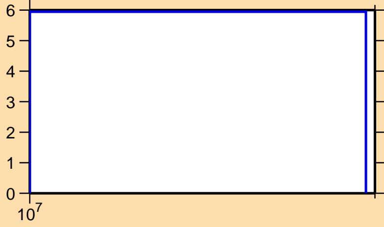
\Delta\sigma/\sigma vs. E for ^{163}\text{Ta}(n,\text{nonel.})
