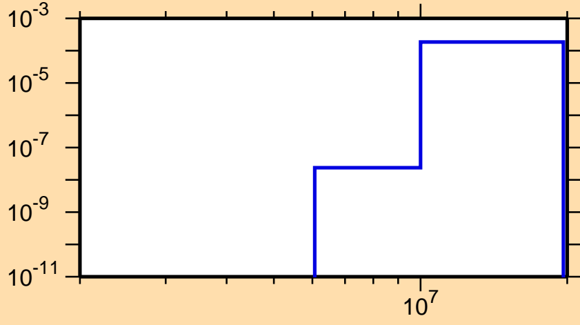
\sigma vs. E for ^{163}\text{Ta} (mt 45)
