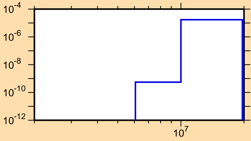
\sigma vs. E for ^{163}\text{Ta}(n,\text{He}3)
