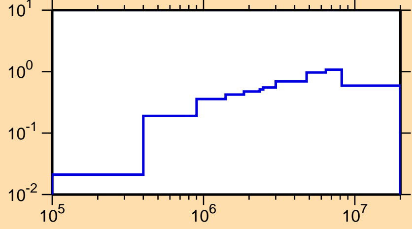
\sigma vs. E for ^{163}\text{Ta}(n,\text{inel.})
