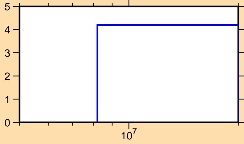
\Delta\sigma/\sigma vs. E for ^{163}\text{Ta}(n,\text{tot.})
