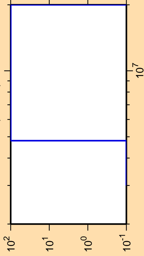
\Delta\sigma/\sigma vs. E for ^{163}\text{Ta}(\text{mt } 45)
