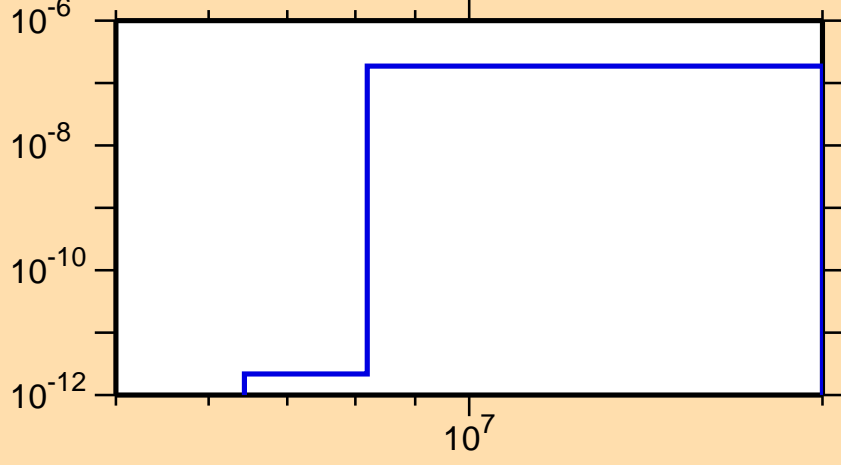
\sigma vs. E for ^{163}\text{Ta}(\text{mt117})
