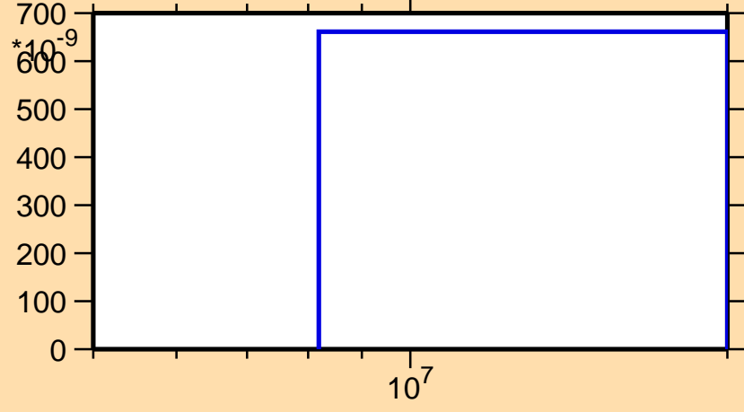
\sigma vs. E for ^{163}\text{Ta}(n,2n\alpha)
