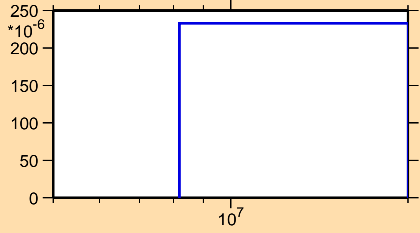
\sigma vs. E for ^{163}\text{Ta}(n,2np)
