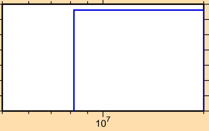
\sigma vs. E for ^{163}\text{Ta}(n,2n\alpha)
