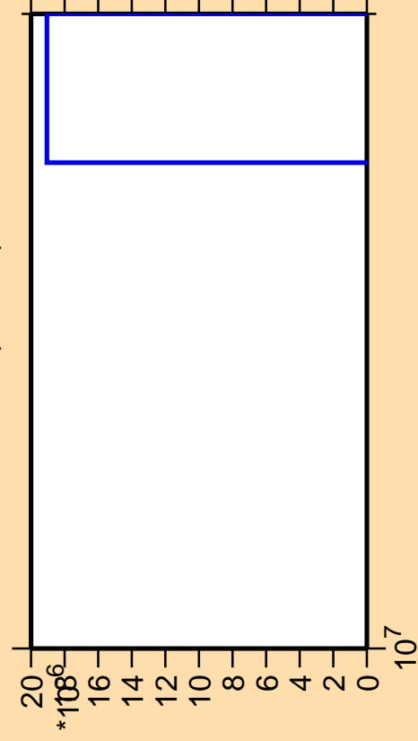
\Delta\sigma/\sigma vs. E for ^{164}\text{Ta} (mt 11)
