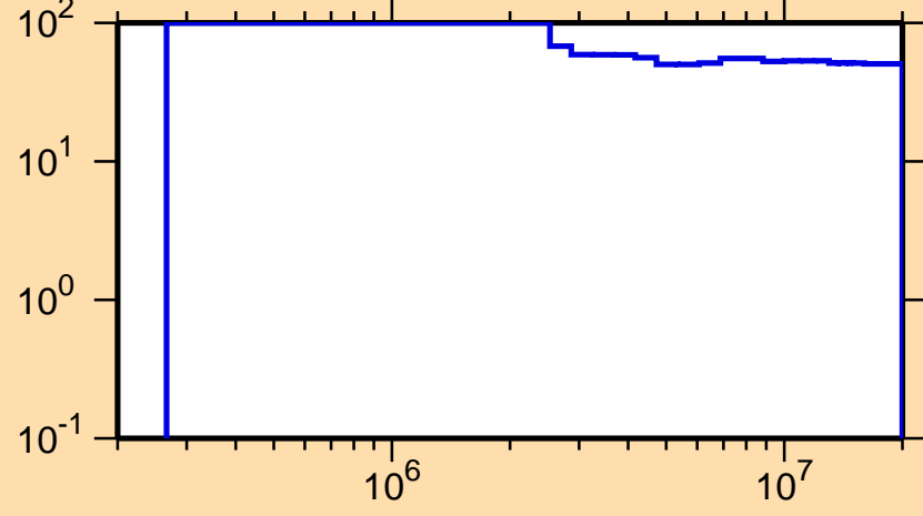
\Delta\sigma/\sigma vs. E for ^{164}\text{Ta}(n,n\text{cont.})
