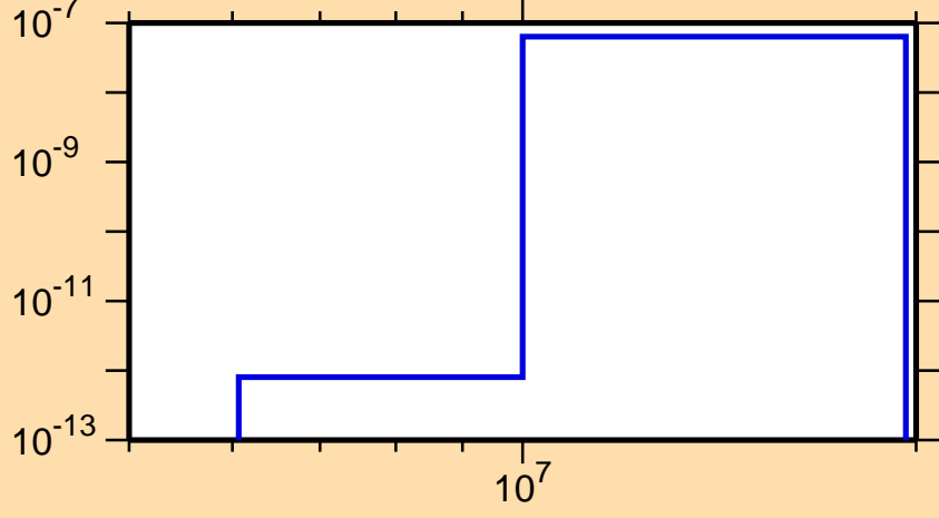
\sigma vs. E for ^{164}\text{Ta}(\text{mt117})
