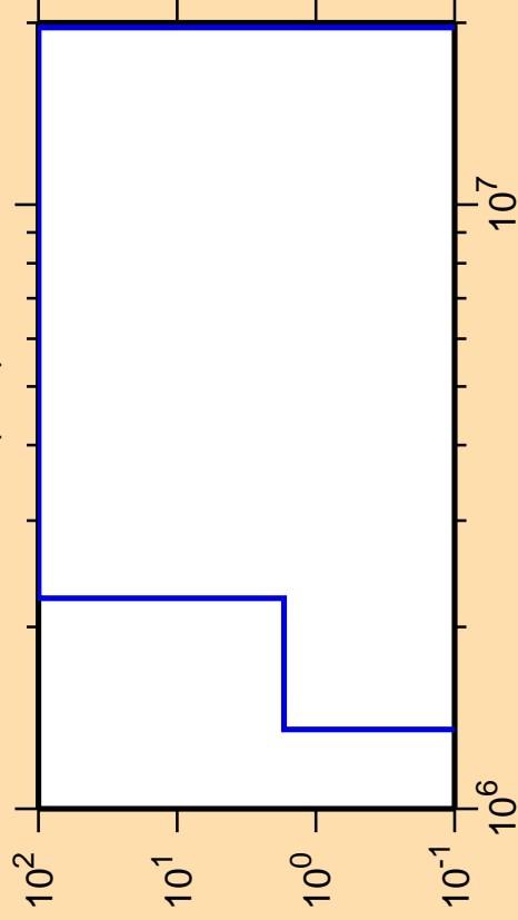
\Delta\sigma/\sigma vs. E for ^{164}\text{Ta}(n,d)
