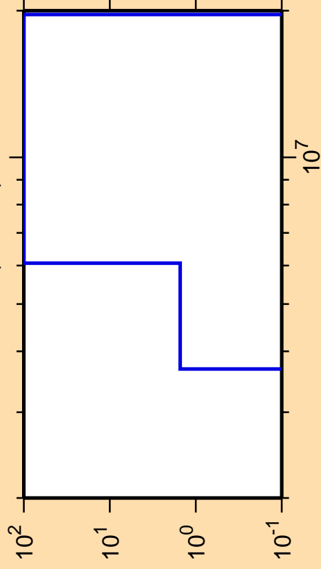
\Delta\sigma/\sigma vs. E for ^{164}\text{Ta}(n,\text{He}3)
