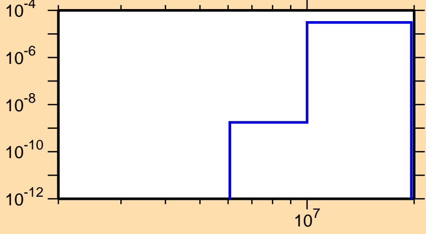
\sigma vs. E for ^{164}\text{Ta}(n,\text{He}3)
