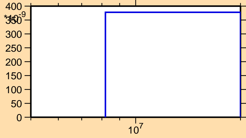
\sigma vs. E for ^{164}\text{Ta}(n,\text{pd})
