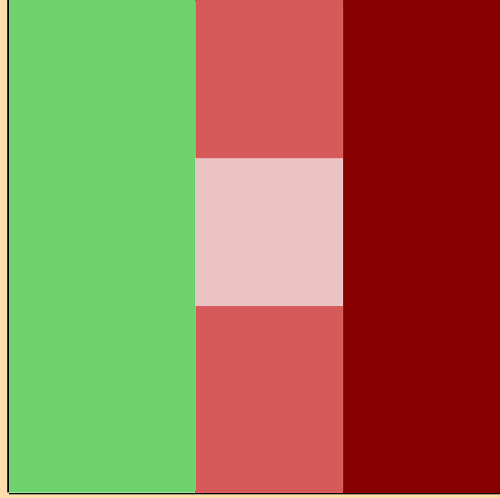
\Delta\sigma/\sigma vs. E for ^{165}\text{Ta}(n,2n)
