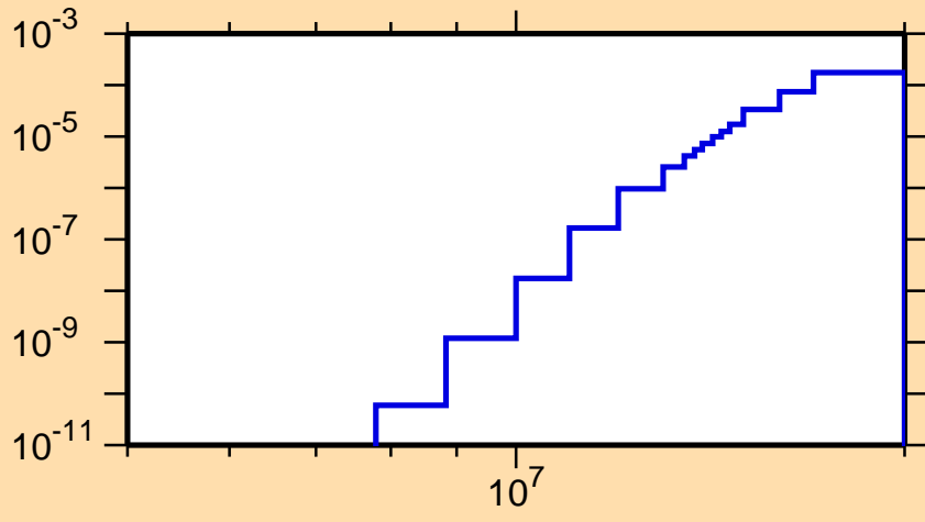
\sigma vs. E for ^{165}\text{Ta}(\text{mt } 45)
