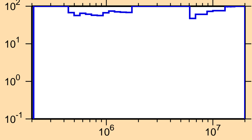
\Delta\sigma/\sigma vs. E for ^{165}\text{Ta}(n,n\text{cont.})
