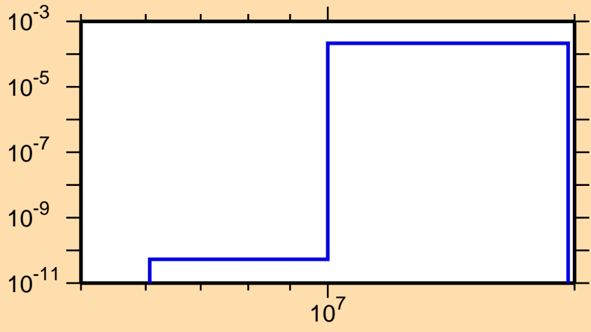
\sigma vs. E for ^{165}\text{Ta}(n,t)
