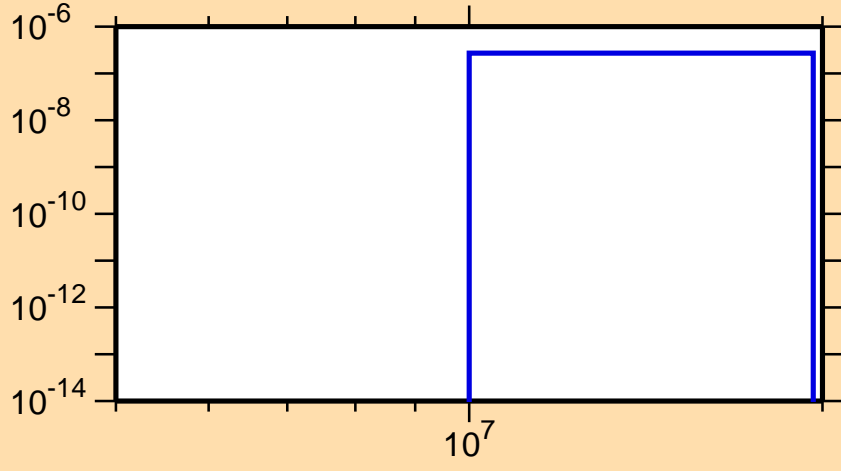
\sigma vs. E for ^{165}\text{Ta}(n,2n\alpha)
