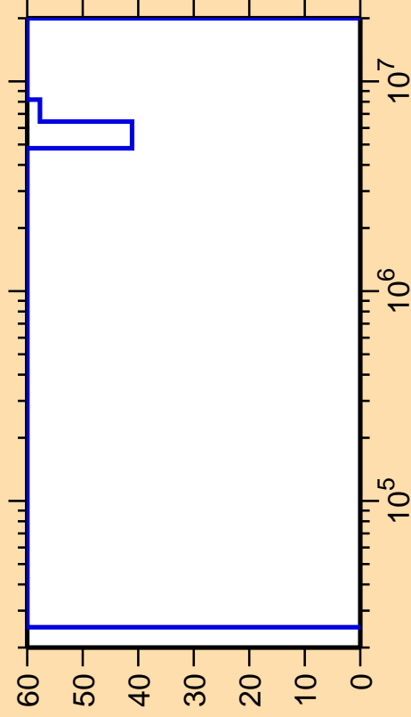
\Delta\sigma/\sigma vs. E for ^{165}\text{Ta}(n,\text{inel.})
