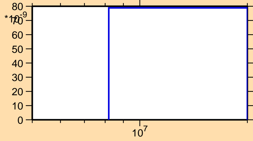
\sigma vs. E for ^{165}\text{Ta}(n,\text{pd})
