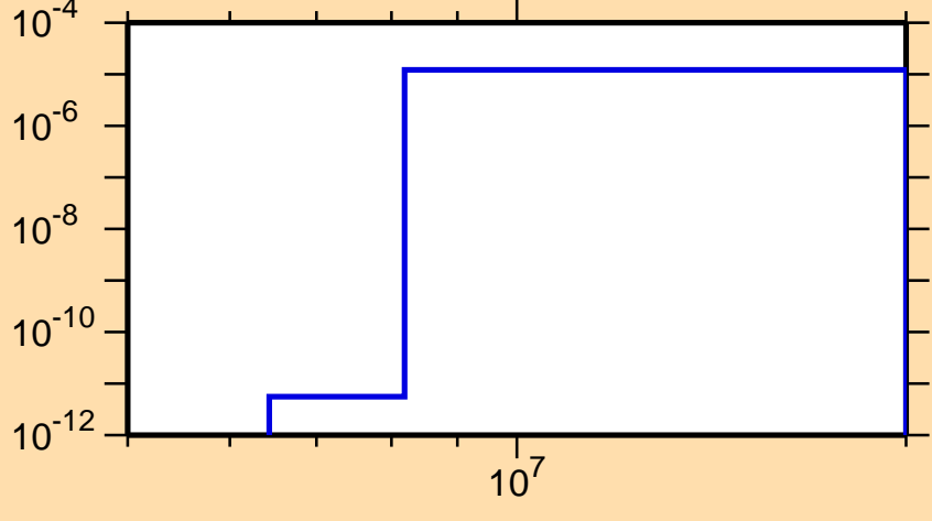
\sigma vs. E for ^{165}\text{Ta}(\text{mt } 45)
