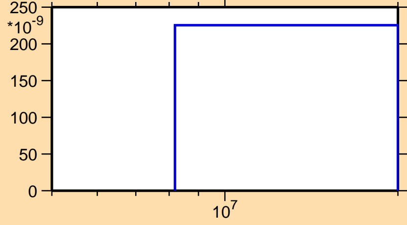
\sigma vs. E for ^{165}\text{Ta}(n,2n\alpha)
