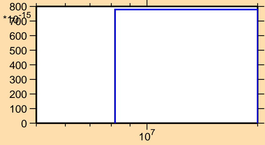
\sigma vs. E for ^{165}\text{Ta}(\text{mt } 34)
