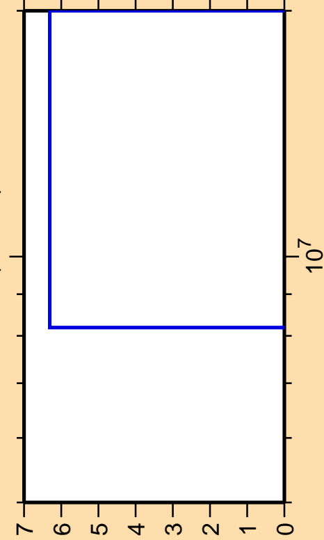
\Delta\sigma/\sigma vs. E for ^{165}\text{Ta}(\text{mt } 34)
