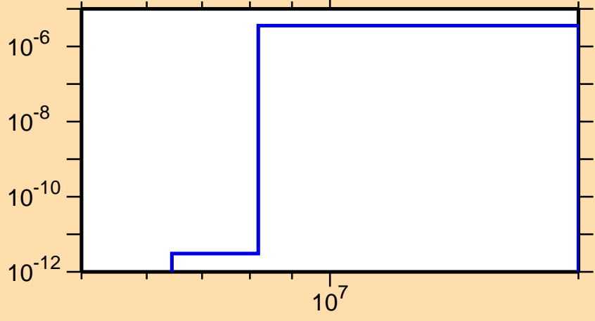
\sigma vs. E for ^{165}\text{Ta}(n,\text{He}3)
