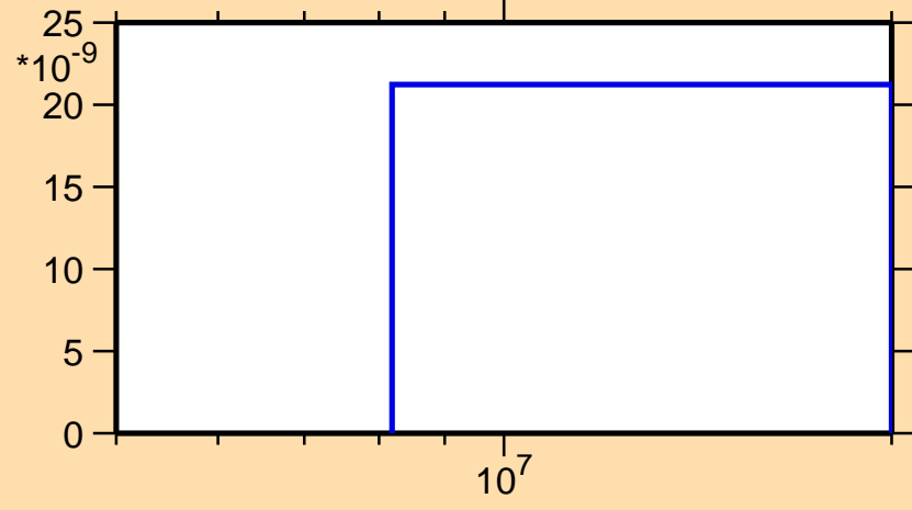
\sigma vs. E for ^{165}\text{Ta}(\text{mt117})
