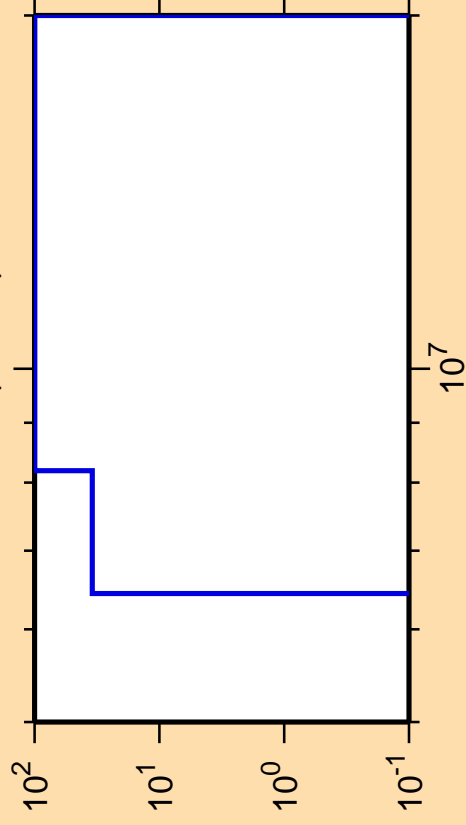
\Delta\sigma/\sigma vs. E for ^{165}\text{Ta}(\text{mt } 45)
