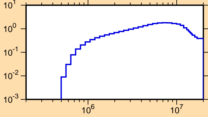
\sigma vs. E for ^{166}\text{Ta}(n,n\text{cont.})
