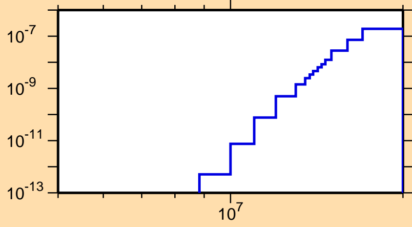
\sigma vs. E for ^{166}\text{Ta}(\text{mt117})
