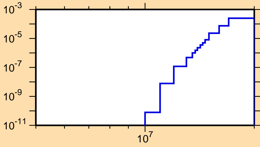
\sigma vs. E for ^{166}\text{Ta}(n,2n\alpha)
