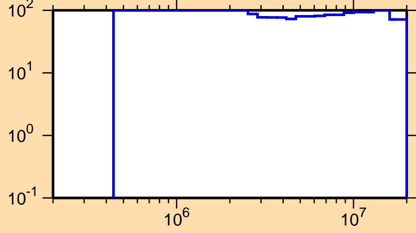
\Delta\sigma/\sigma vs. E for ^{166}\text{Ta}(n,n\text{cont.})
