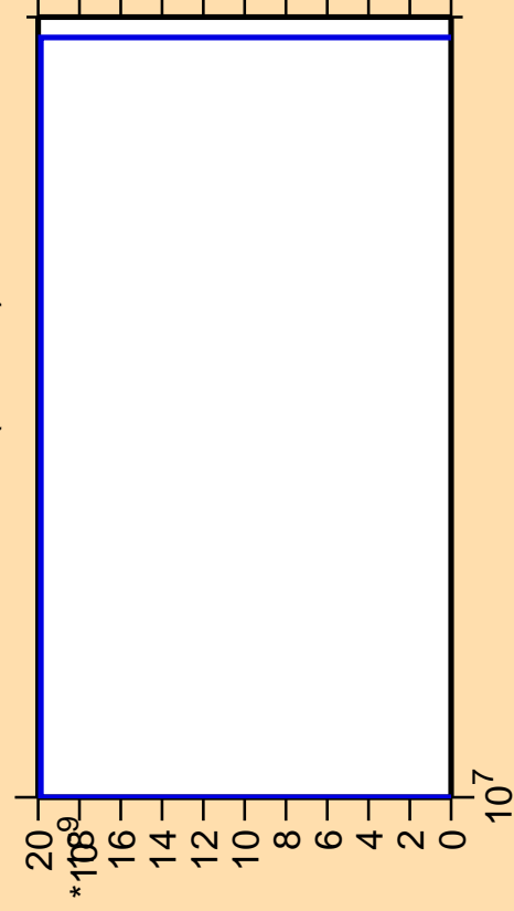
\Delta\sigma/\sigma vs. E for ^{166}\text{Ta} (mt 11)
