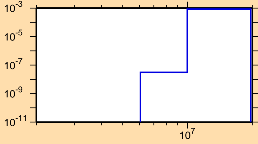
\sigma vs. E for ^{166}\text{Ta}(n,t)
