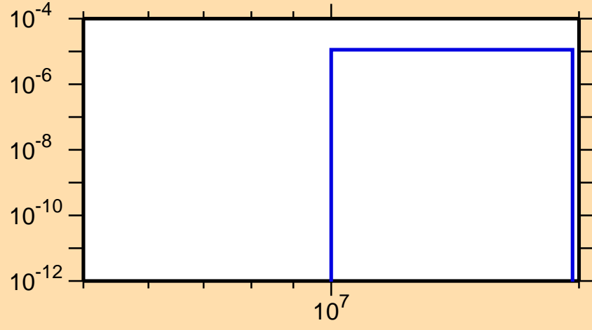
\sigma vs. E for ^{166}\text{Ta}(n,2n\alpha)
