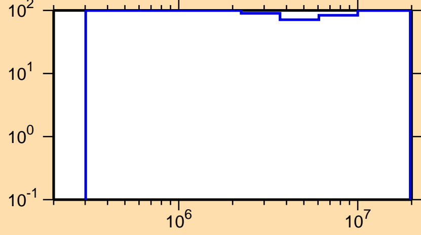
\Delta\sigma/\sigma vs. E for ^{166}\text{Ta}(n,ncont.)
