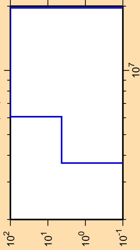
\Delta\sigma/\sigma vs. E for ^{166}\text{Ta}(n,t)
