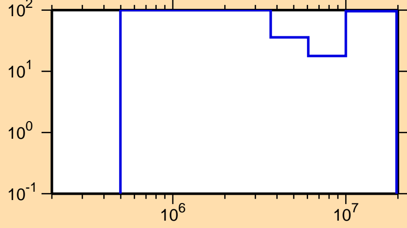
\Delta\sigma/\sigma vs. E for ^{167}\text{Ta}(n,ncont.)
