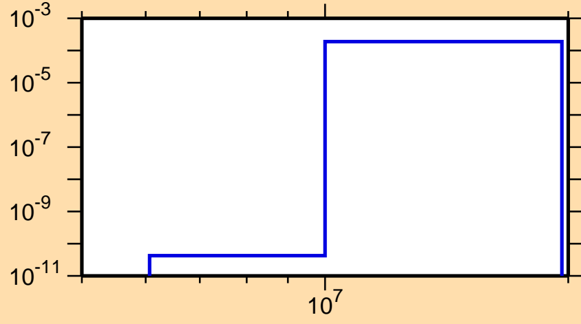
\sigma vs. E for ^{167}\text{Ta}(n,t)
