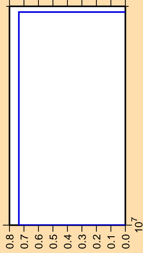
\Delta\sigma/\sigma vs. E for ^{167}\text{Ta} (mt 34)
