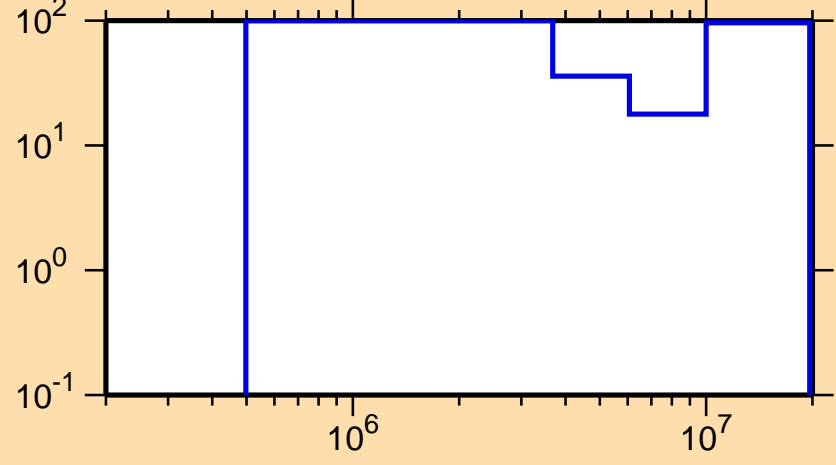
\Delta\sigma/\sigma vs. E for ^{167}\text{Ta}(n,n\text{cont.})
