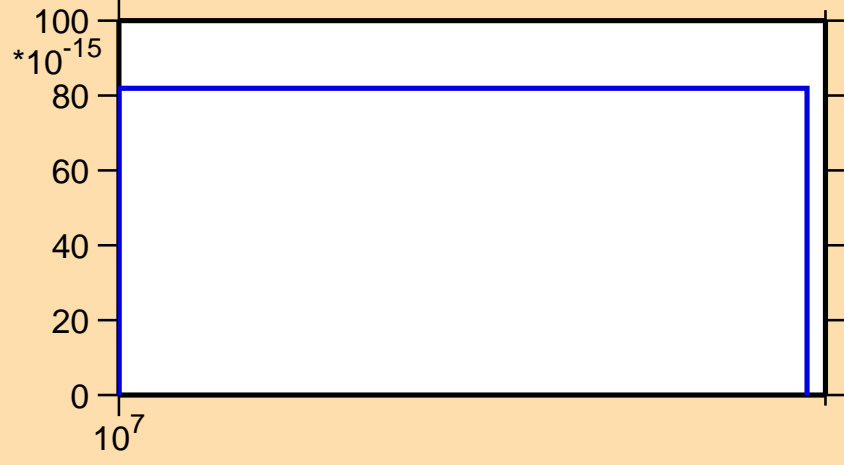
\sigma vs. E for ^{167}\text{Ta} (mt 34)
