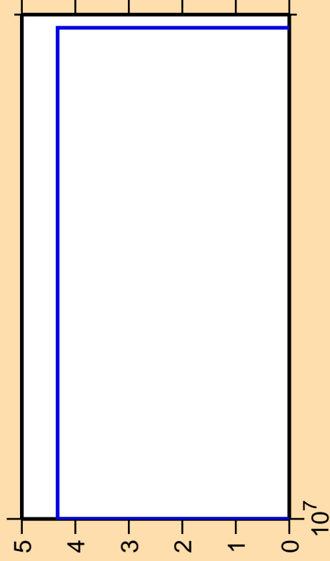
\Delta\sigma/\sigma vs. E for ^{167}\text{Ta}(n,\text{pt})
