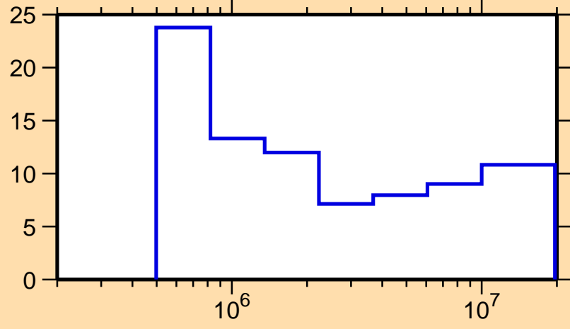
\Delta\sigma/\sigma vs. E for ^{167}\text{Ta}(n,nonel.)
