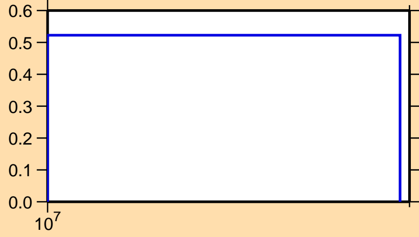
\sigma vs. E for ^{167}\text{Ta}(n,2n)
