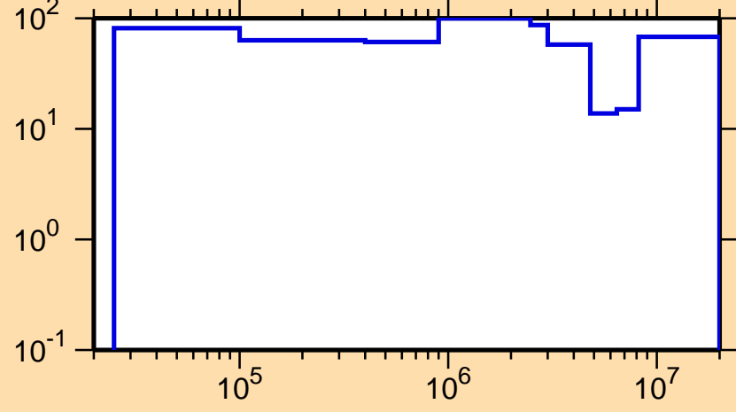
\Delta\sigma/\sigma vs. E for ^{167}\text{Ta}(n,\text{inel.})
