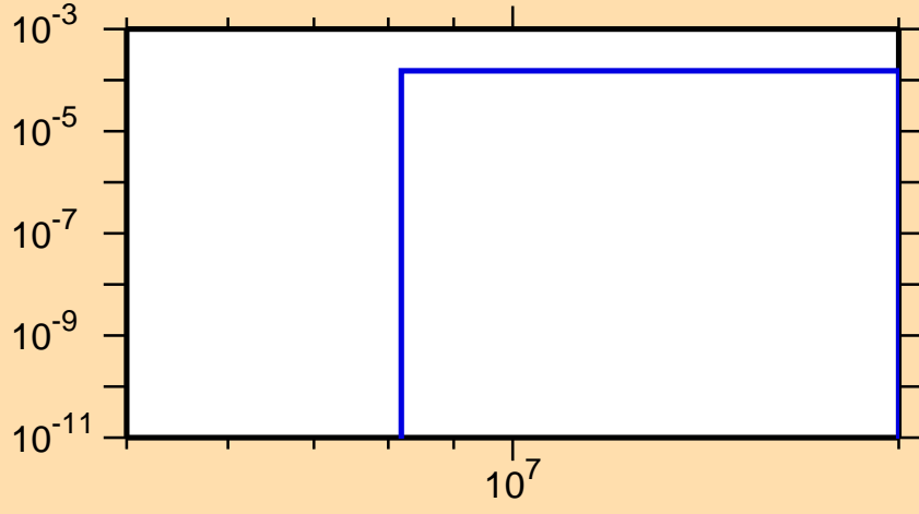
\sigma vs. E for ^{167}\text{Ta}(n,t)
