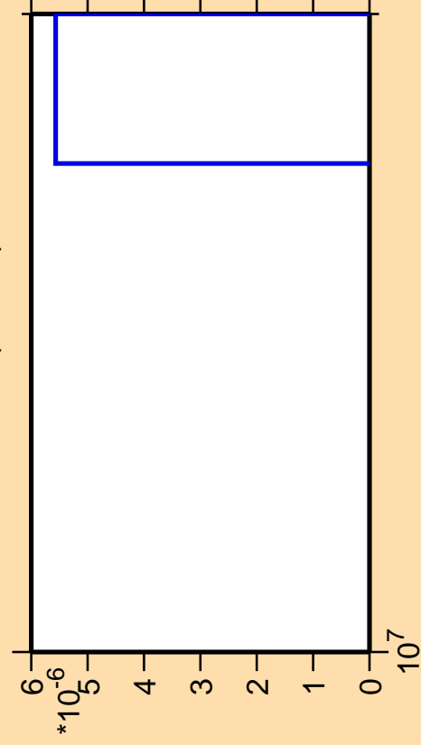
\Delta\sigma/\sigma vs. E for ^{168}\text{Ta} (mt 11)
