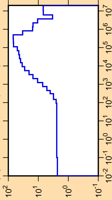
\Delta\mu/\mu vs. E for ^{168}\text{Ta}(\text{mt251})
