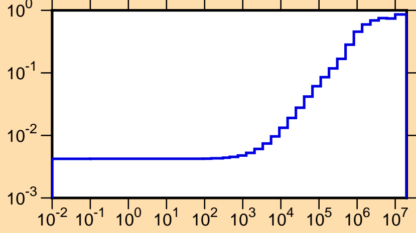
\mu vs. E for ^{168}\text{Ta}(\text{mt251})
