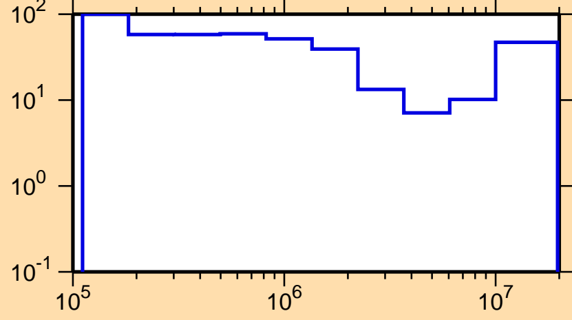
\Delta\sigma/\sigma vs. E for ^{168}\text{Ta}(n,\text{inel.})
