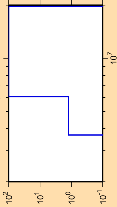
\Delta\sigma/\sigma vs. E for ^{168}\text{Ta}(n,t)
