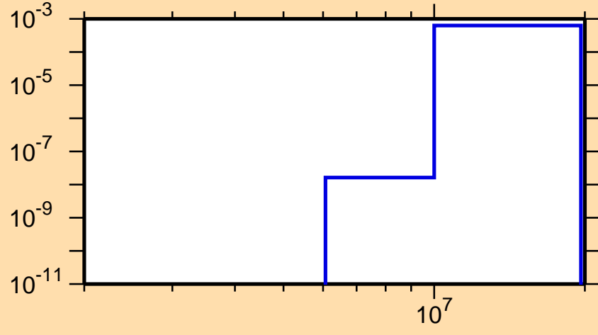
\sigma vs. E for ^{168}\text{Ta}(n,t)
