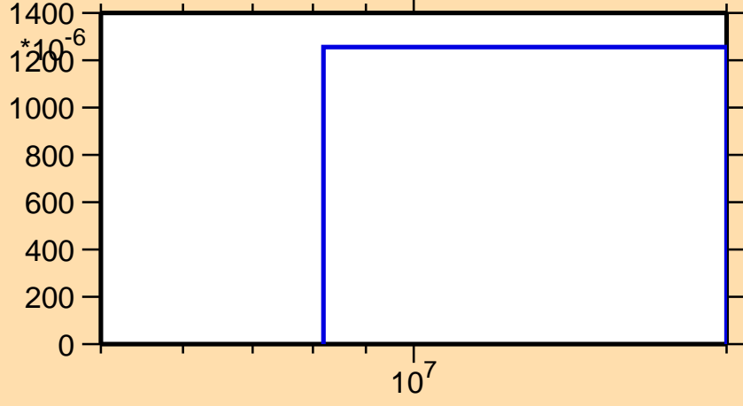
\sigma vs. E for ^{168}\text{Ta}(n,2np)
