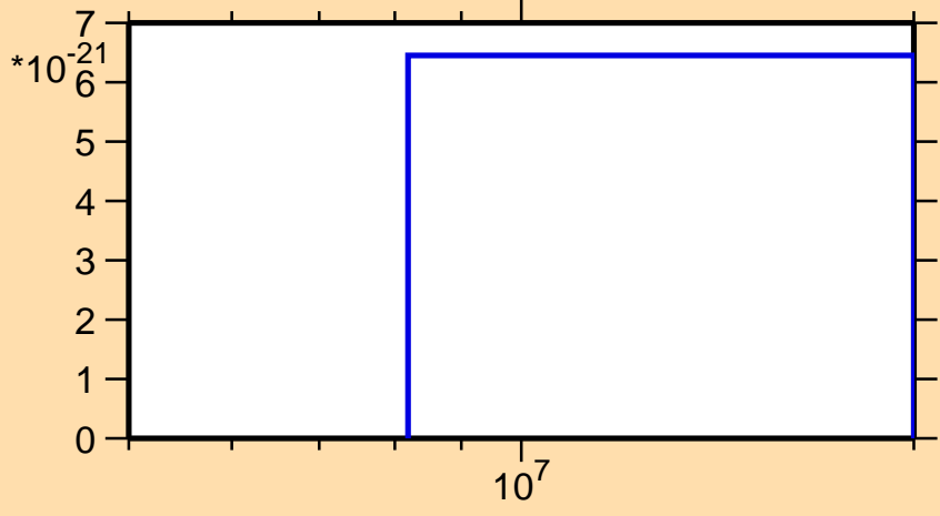
\sigma vs. E for ^{168}\text{Ta}(\text{mt } 11)
