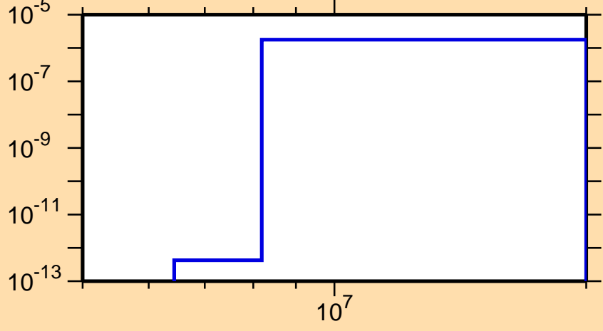
\sigma vs. E for ^{168}\text{Ta}(n,\text{He3})
