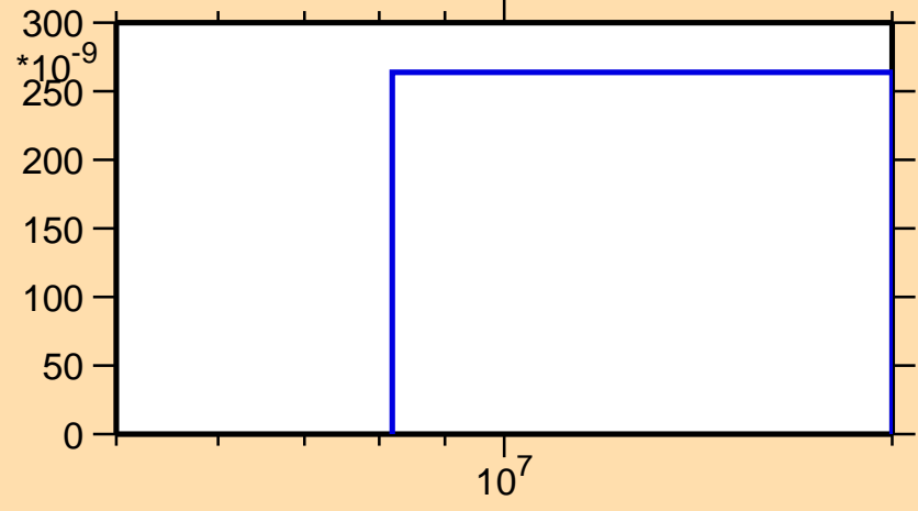
\sigma vs. E for ^{168}\text{Ta}(\text{mt } 45)
