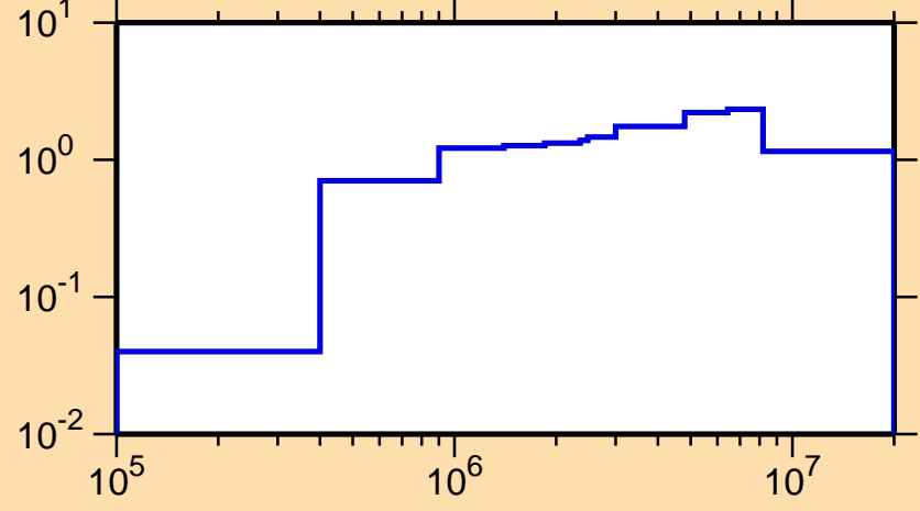
\sigma vs. E for ^{168}\text{Ta}(n,\text{inel.})
