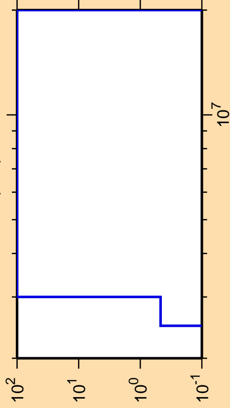
\Delta\sigma/\sigma vs. E for ^{168}\text{Ta}(n,d)
