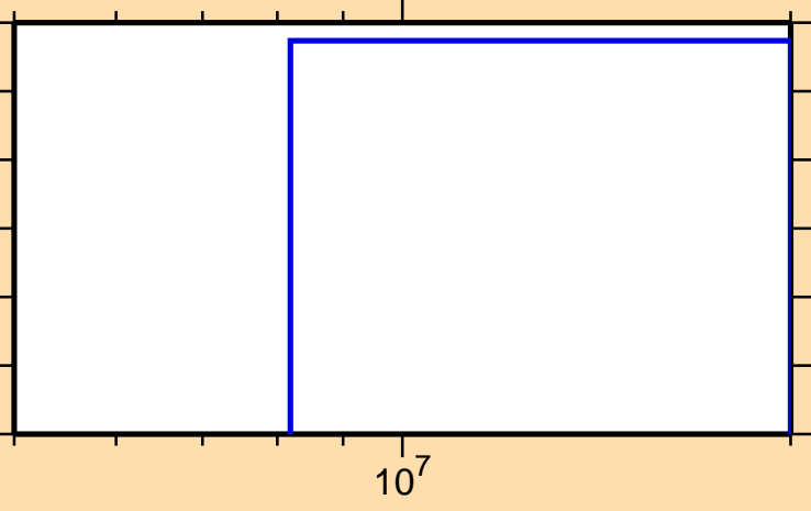
\sigma vs. E for ^{168}\text{Ta}(n,nt)
