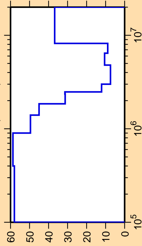
\Delta\sigma/\sigma vs. E for ^{168}\text{Ta}(n,\text{inel.})
