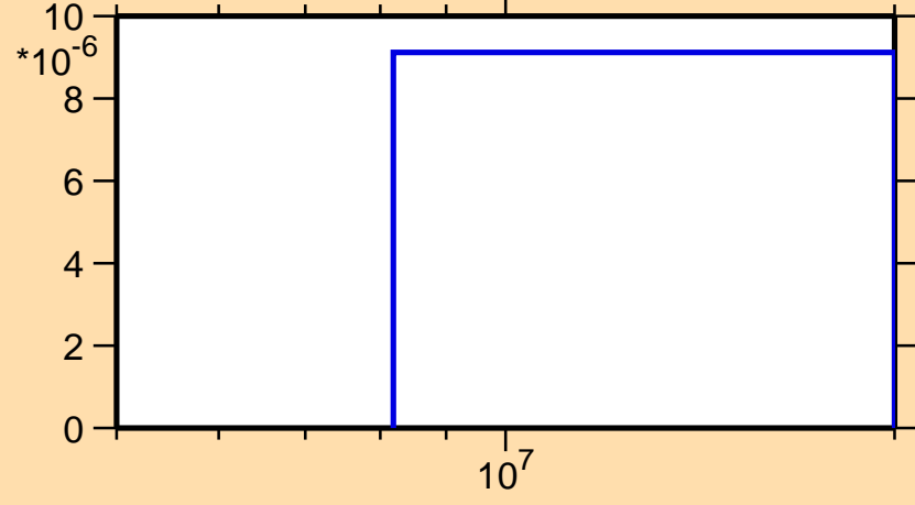
\sigma vs. E for ^{168}\text{Ta}(n,2n\alpha)
