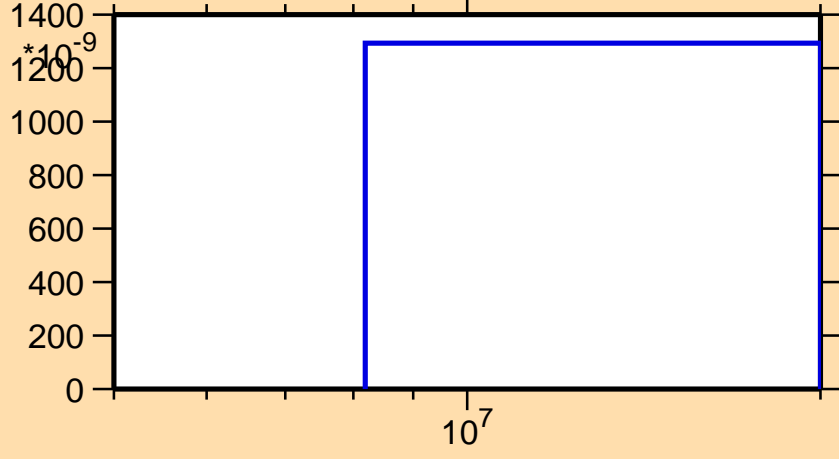
\sigma vs. E for ^{168}\text{Ta}(n,3n)
