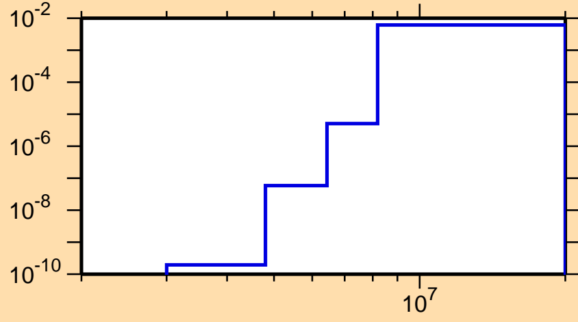
\sigma vs. E for ^{168}\text{Ta}(n,d)
