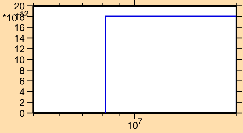
\sigma vs. E for ^{168}\text{Ta}(\text{mt } 34)
