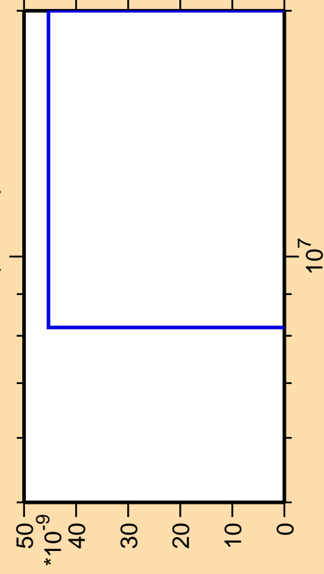
\Delta\sigma/\sigma vs. E for ^{168}\text{Ta}(\text{mt } 11)
