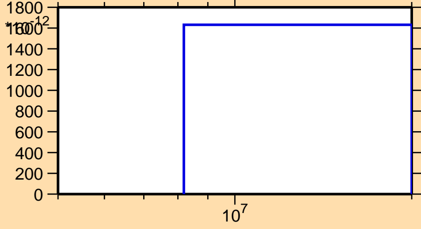
\sigma vs. E for ^{168}\text{Ta}(n,\text{pd})
