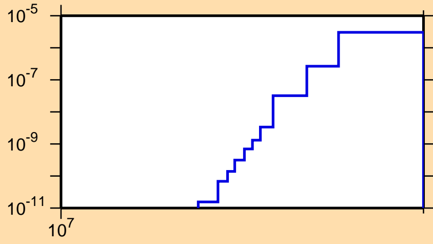
\sigma vs. E for ^{169}\text{Ta}(n,2n\alpha)
