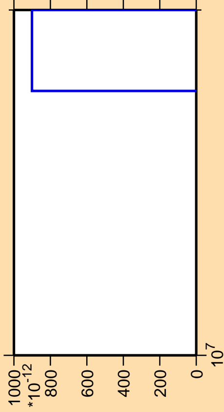
\Delta\sigma/\sigma vs. E for ^{169}\text{Ta} (mt 42)
