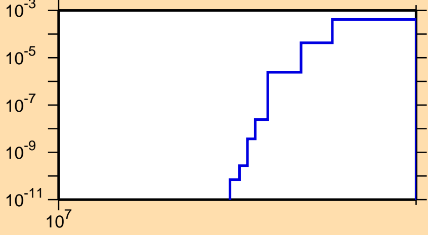
\sigma vs. E for ^{169}\text{Ta}(n,2np)
