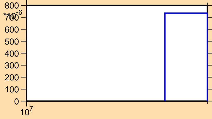
\sigma vs. E for ^{169}\text{Ta}(n,3n)
