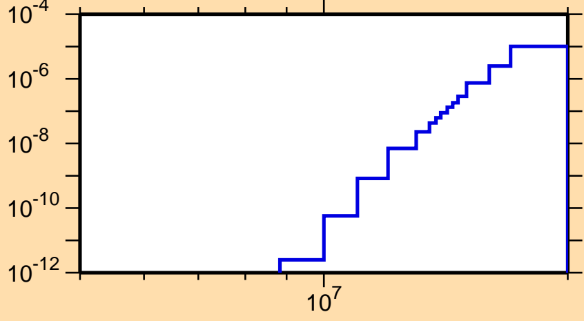
\sigma vs. E for ^{169}\text{Ta}(n,\text{He}3)
