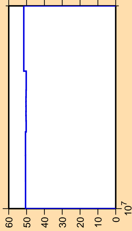
\Delta\sigma/\sigma vs. E for ^{169}\text{Ta}(n,n_1)
