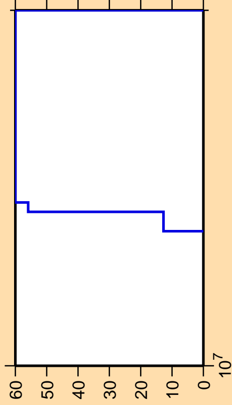
\Delta\sigma/\sigma vs. E for ^{169}\text{Ta}(n,2n\alpha)
