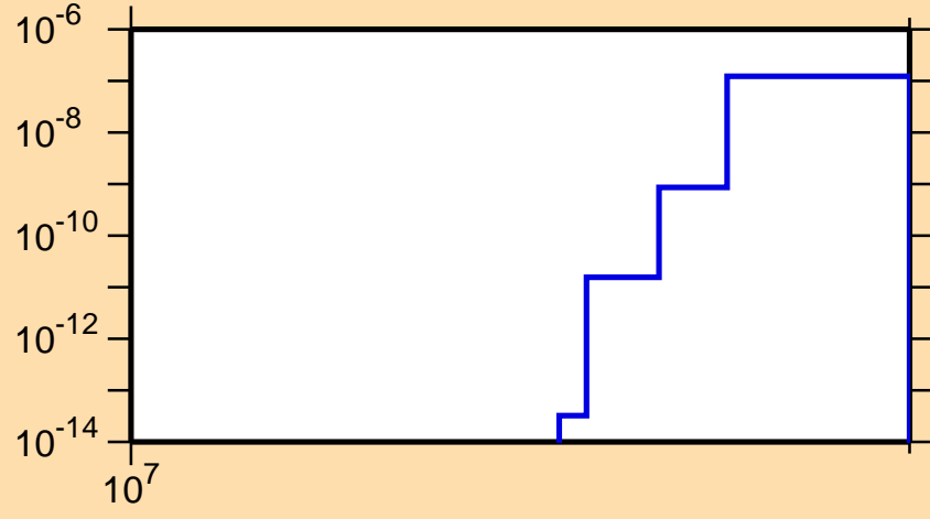
\sigma vs. E for ^{169}\text{Ta}(n,nt)
