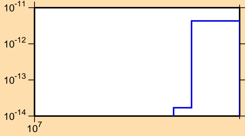
\sigma vs. E for ^{169}\text{Ta} (mt 34)
