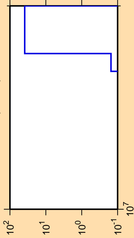
\Delta\sigma/\sigma vs. E for ^{169}\text{Ta} (mt 34)
