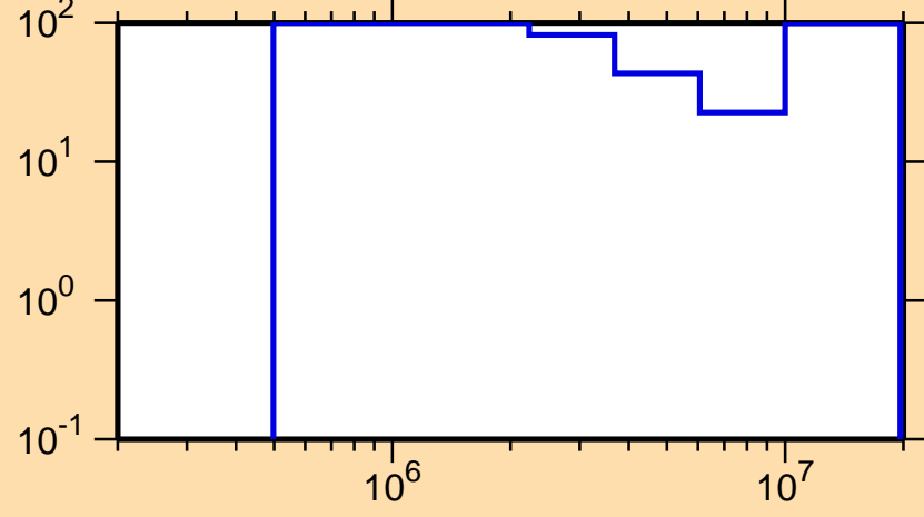
\Delta\sigma/\sigma vs. E for ^{169}\text{Ta}(n,n\text{cont.})
