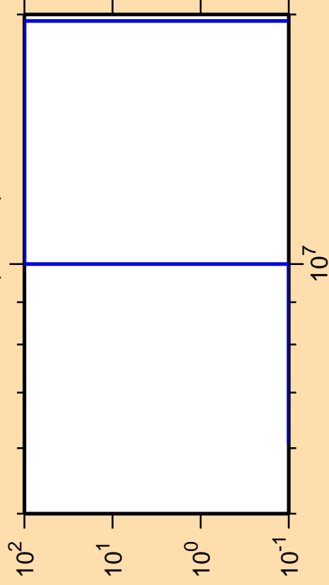
\Delta\sigma/\sigma vs. E for ^{169}\text{Ta}(\text{mt } 45)
