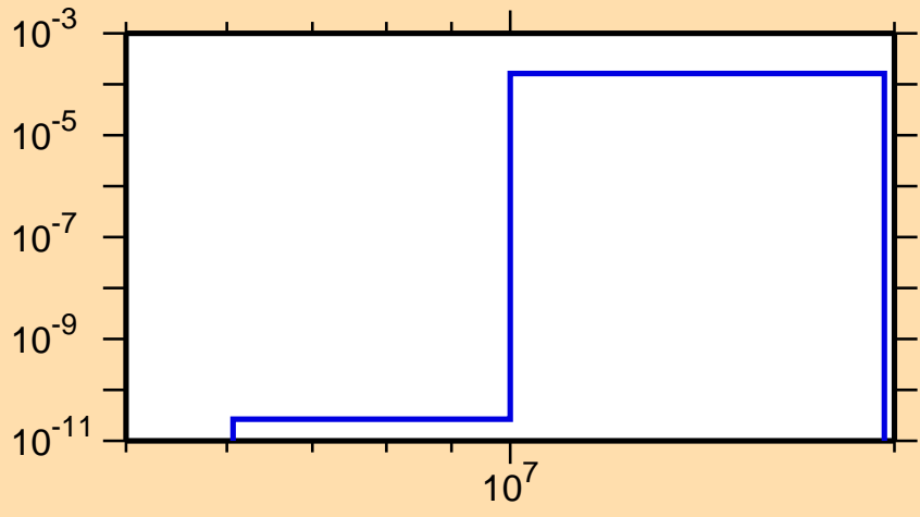
\sigma vs. E for ^{169}\text{Ta}(n,t)
