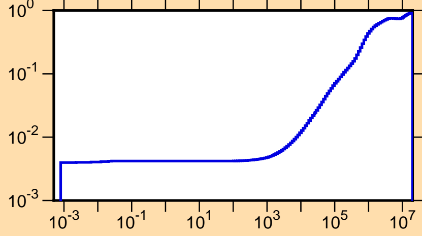
\mu vs. E for ^{170}\text{Ta}(\text{mt251})
