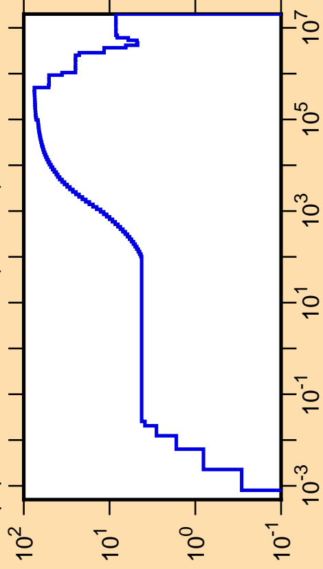
\Delta\mu/\mu vs. E for ^{170}\text{Ta}(\text{mt251})
