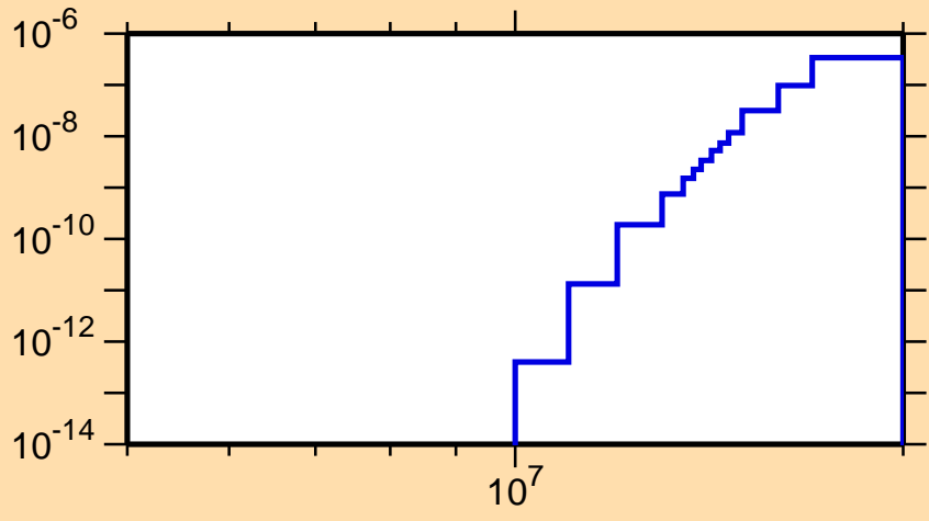
\sigma vs. E for ^{170}\text{Ta} (mt 45)
