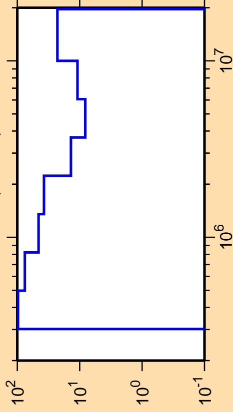
\Delta\sigma/\sigma vs. E for ^{170}\text{Ta}(n,\text{inel.})
