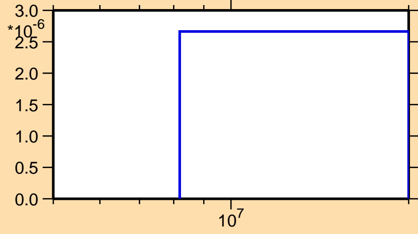
\sigma vs. E for ^{170}\text{Ta}(n,2n\alpha)
