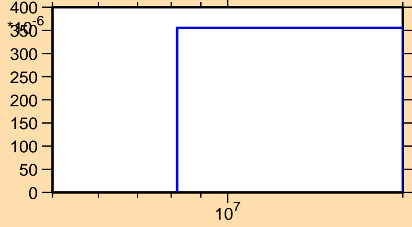
\sigma vs. E for ^{170}\text{Ta}(n,2np)
