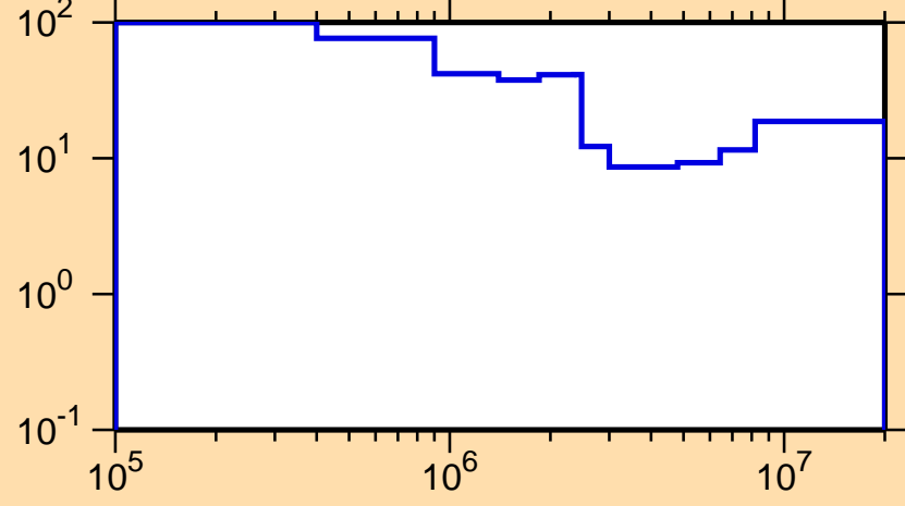
\Delta\sigma/\sigma vs. E for ^{170}\text{Ta}(n,\text{inel.})
