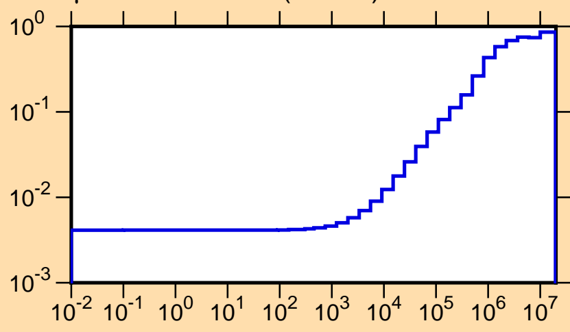
\mu vs. E for ^{171}\text{Ta}(\text{mt251})
