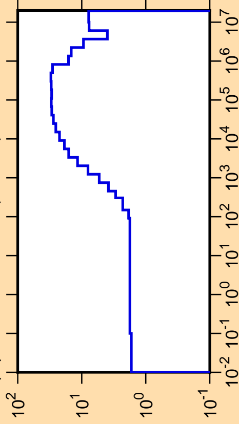
\Delta\mu/\mu vs. E for ^{171}\text{Ta}(\text{mt251})
