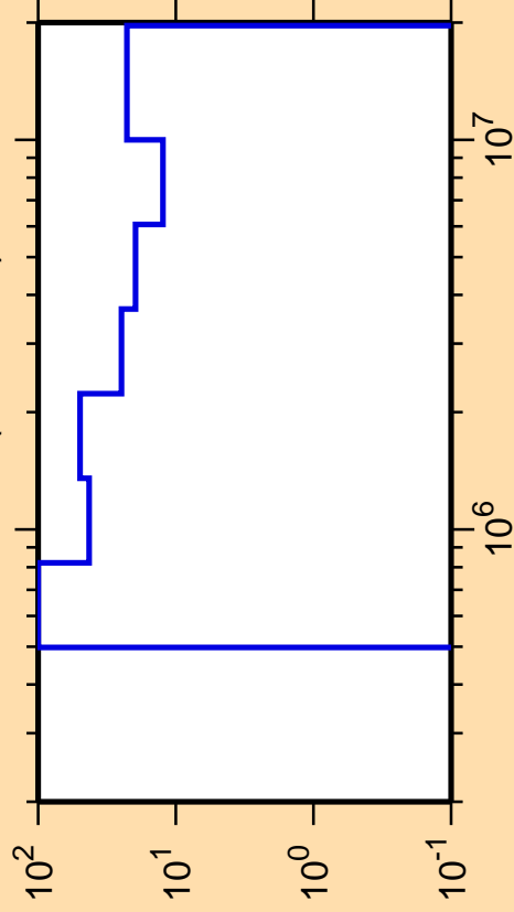
\Delta\sigma/\sigma vs. E for ^{171}\text{Ta}(n,\text{ncont.})
