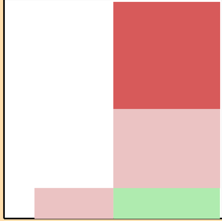
\Delta\sigma/\sigma vs. E for ^{171}\text{Ta}(n,2n)
