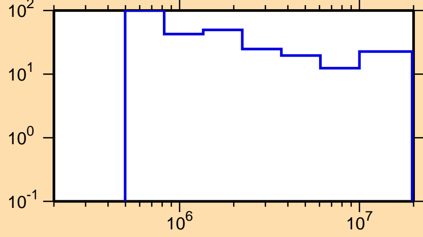
\Delta\sigma/\sigma vs. E for ^{171}\text{Ta}(n,ncont.)
