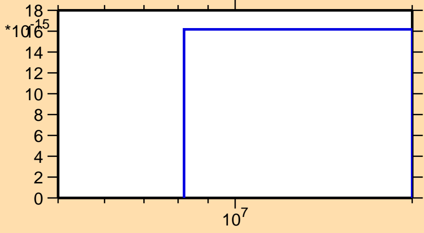
\sigma vs. E for ^{171}\text{Ta} (mt 34)
