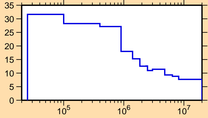
\Delta\sigma/\sigma vs. E for ^{171}\text{Ta}(n,\text{nonel.})
