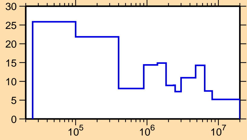
\Delta\sigma/\sigma vs. E for ^{171}\text{Ta}(n,\text{el.})
