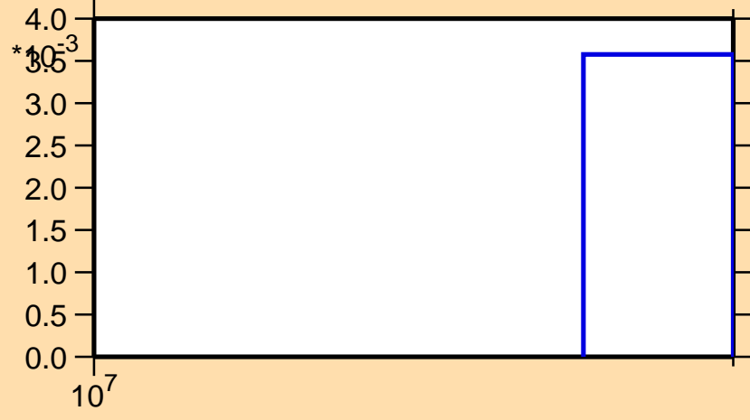
\sigma vs. E for ^{172}\text{Ta}(n,3n)
