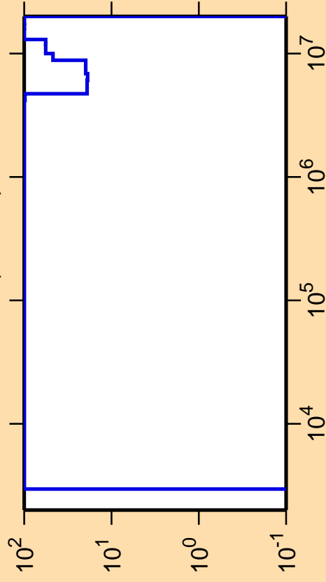
\Delta\sigma/\sigma vs. E for ^{172}\text{Ta}(n,\text{inel.})
