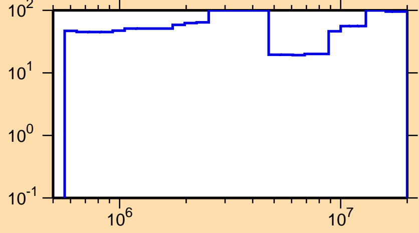
\Delta\sigma/\sigma vs. E for ^{172}\text{Ta}(n,n\text{cont.})
