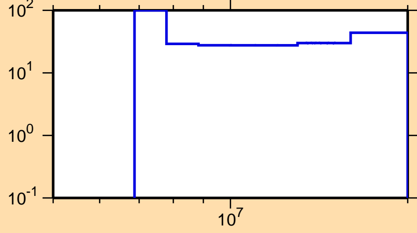
\Delta\sigma/\sigma vs. E for ^{172}\text{Ta}(n,2n)
