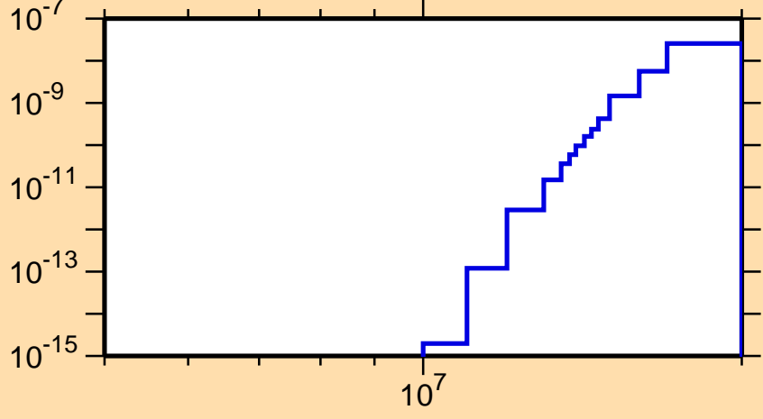
\sigma vs. E for ^{172}\text{Ta} (mt 45)
