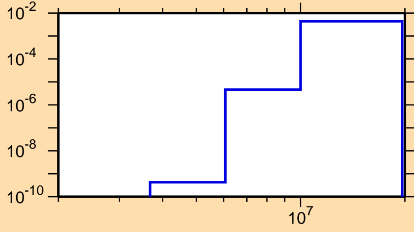
\sigma vs. E for ^{172}\text{Ta}(n,d)
