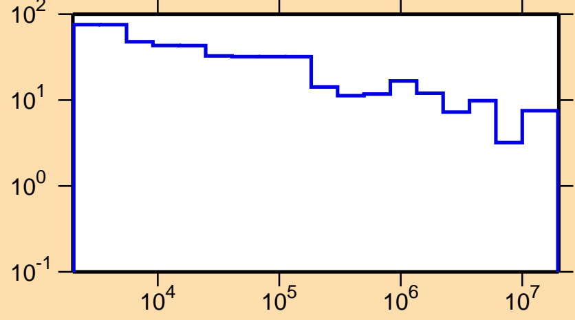
\Delta\sigma/\sigma vs. E for ^{172}\text{Ta}(n,\text{tot.})
