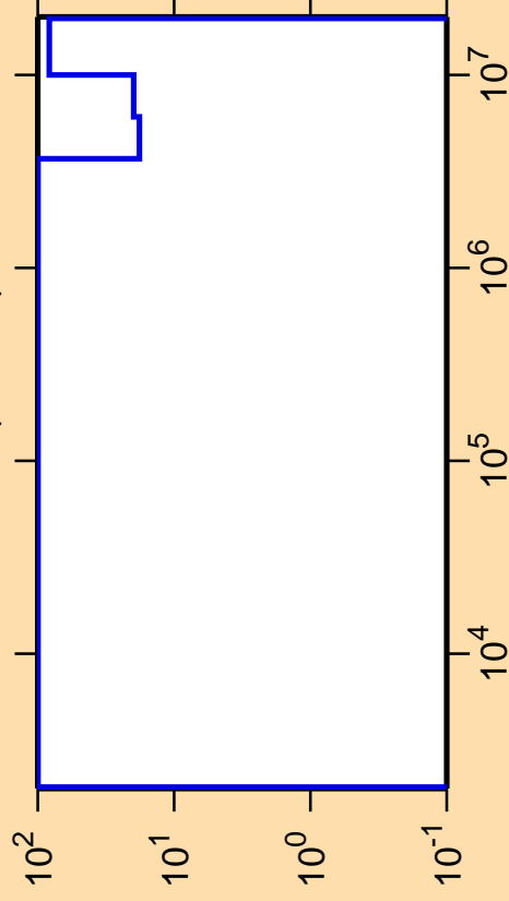
\Delta\sigma/\sigma vs. E for ^{172}\text{Ta}(n,\text{inel.})
