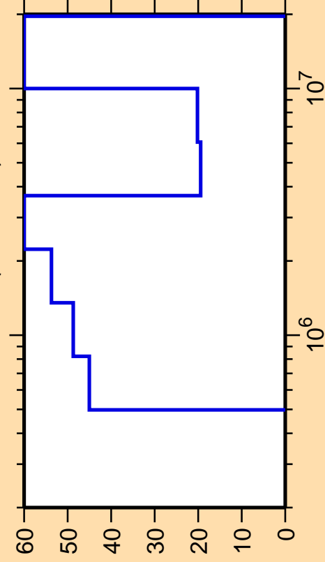
\Delta\sigma/\sigma vs. E for ^{172}\text{Ta}(n,\text{ncont.})
