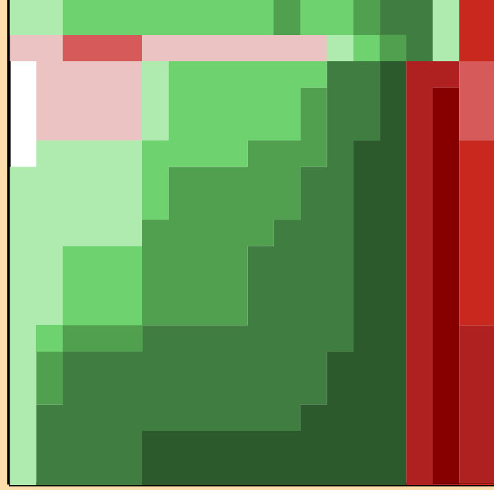
\Delta\sigma/\sigma vs. E for ^{172}\text{Ta}(n,\text{inel.})
