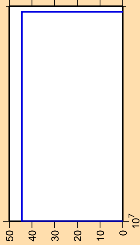
\Delta\sigma/\sigma vs. E for ^{172}\text{Ta}(n,\text{pd})
