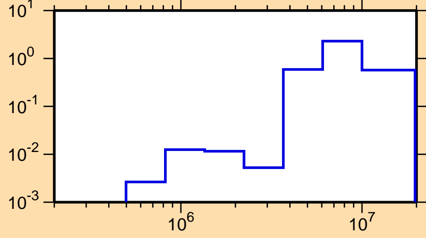
\sigma vs. E for ^{172}\text{Ta}(n,n\text{cont.})
