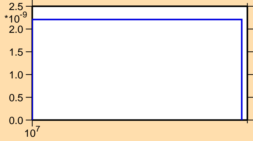
\sigma vs. E for ^{172}\text{Ta}(n,nt)
