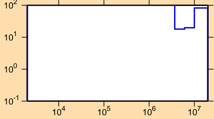
\Delta\sigma/\sigma vs. E for ^{172}\text{Ta}(n,\text{inel.})
