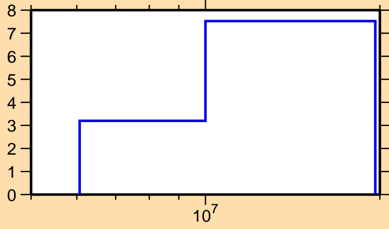
\Delta\sigma/\sigma vs. E for ^{172}\text{Ta}(n,\text{tot.})
