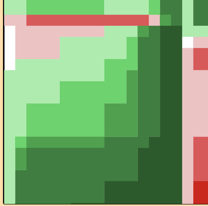
\Delta\sigma/\sigma vs. E for ^{172}\text{Ta}(n,n_1)
