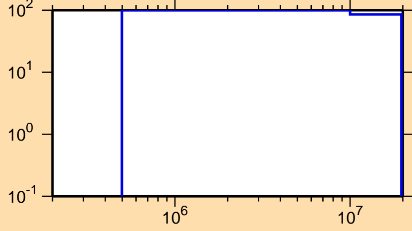
\Delta\sigma/\sigma vs. E for ^{172}\text{Ta}(n,n_1)
