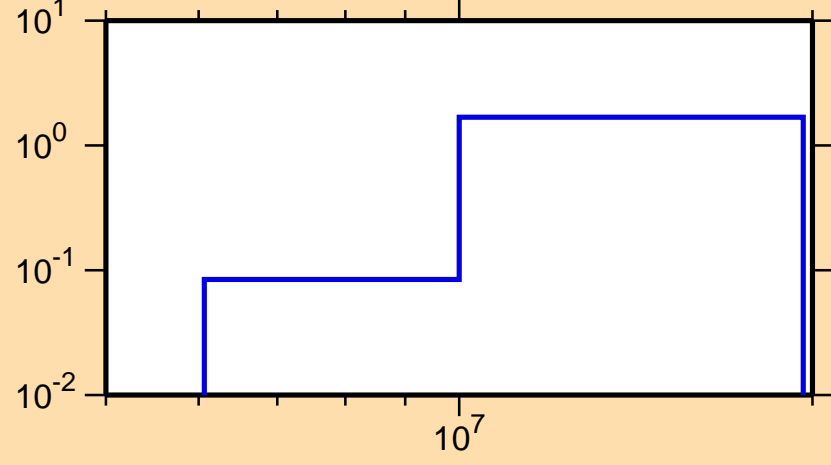
\sigma vs. E for ^{172}\text{Ta}(n,2n)
