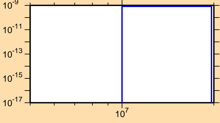
\sigma vs. E for ^{172}\text{Ta}(\text{mt } 45)
