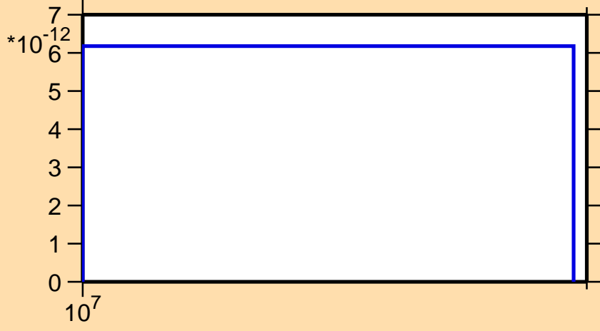
\sigma vs. E for ^{172}\text{Ta}(n,\text{pd})
