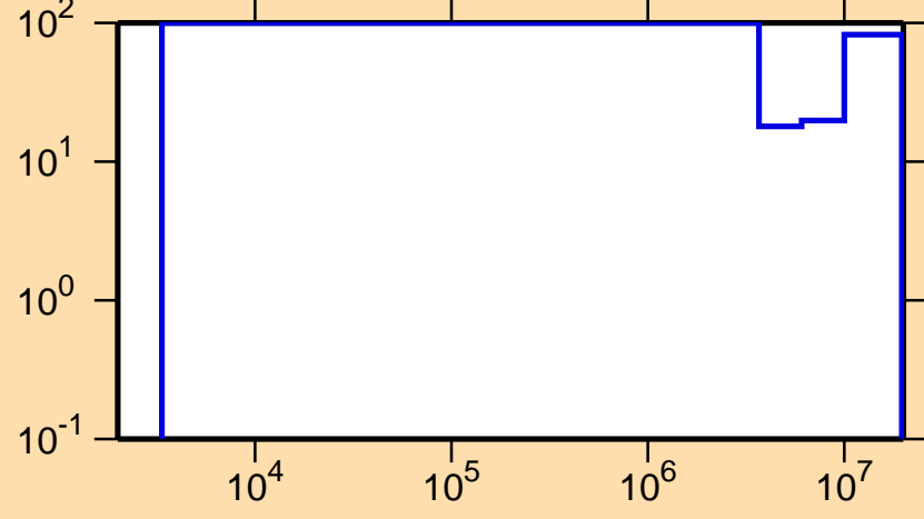
\Delta\sigma/\sigma vs. E for ^{172}\text{Ta}(n,\text{inel.})
