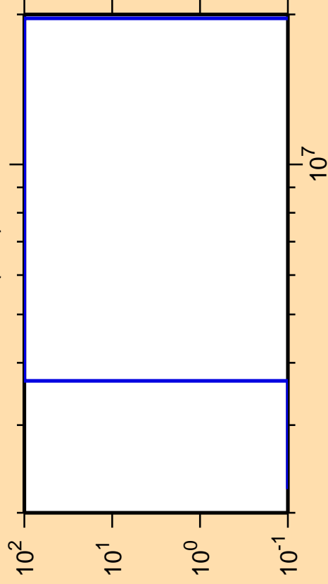
\Delta\sigma/\sigma vs. E for ^{172}\text{Ta}(n,d)
