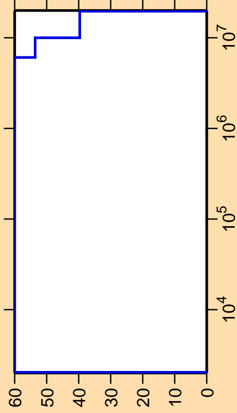
\Delta\sigma/\sigma vs. E for ^{172}\text{Ta}(n,p)
