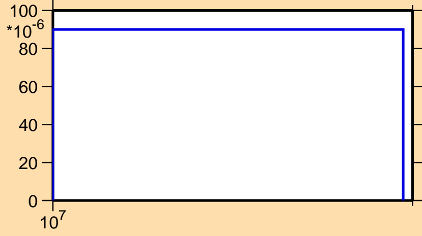
\sigma vs. E for ^{172}\text{Ta}(n,2np)
