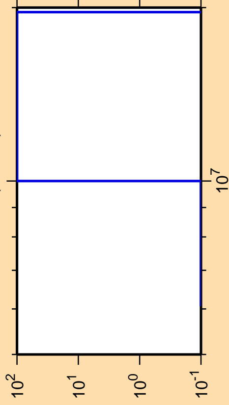
\Delta\sigma/\sigma vs. E for ^{172}\text{Ta}(\text{mt } 45)
