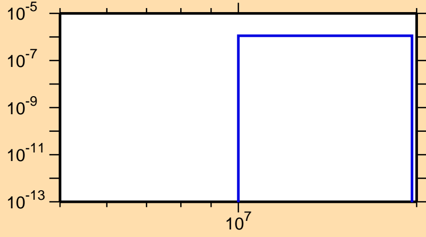
\sigma vs. E for ^{172}\text{Ta}(n,2n\alpha)
