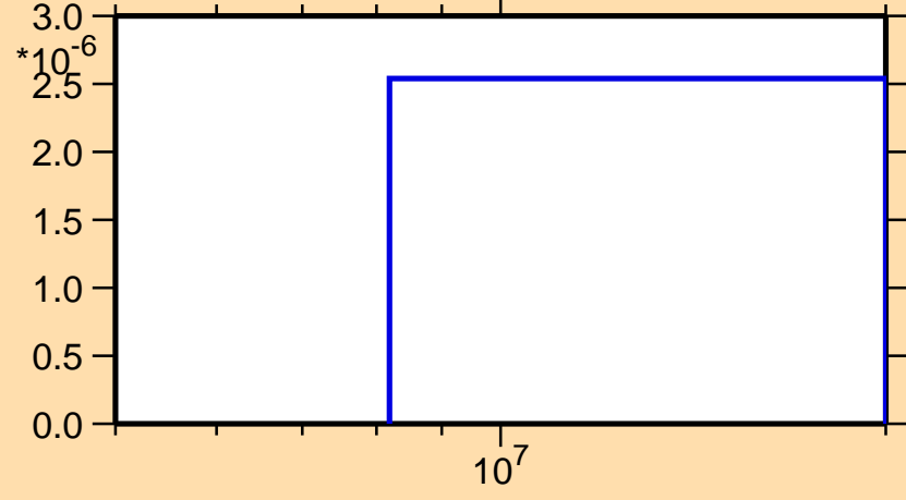
\sigma vs. E for ^{172}\text{Ta}(n,\text{nd})
