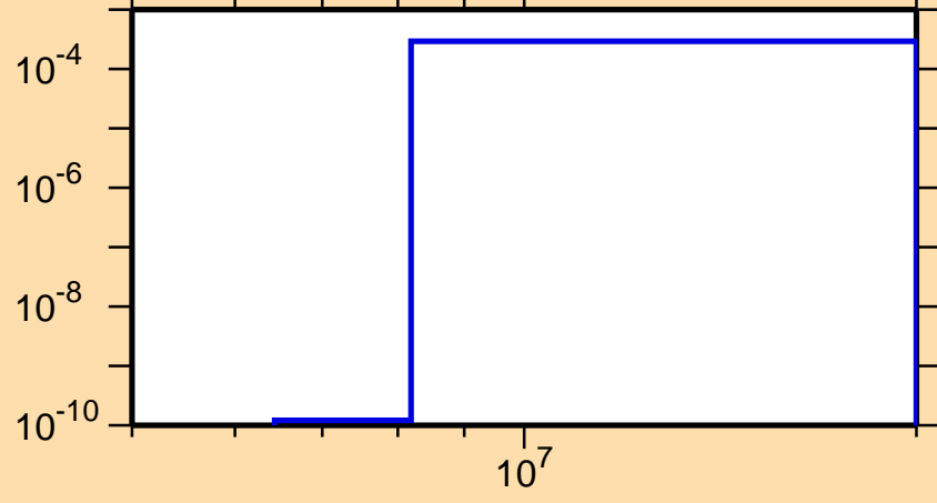
\sigma vs. E for ^{172}\text{Ta}(n,t)
