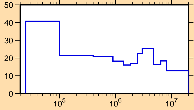
\Delta\sigma/\sigma vs. E for ^{173}\text{Ta}(n,\text{el.})
