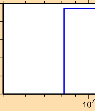
\sigma vs. E for ^{173}\text{Ta}(n,nt)
