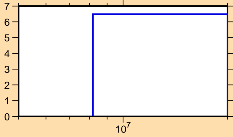
\Delta\sigma/\sigma vs. E for ^{173}\text{Ta}(n,\text{nonel.})
