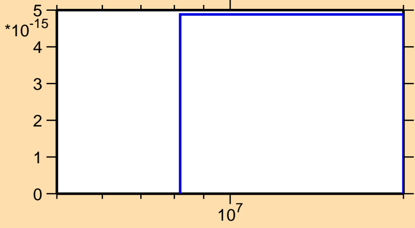
\sigma vs. E for ^{173}\text{Ta} (mt 34)
