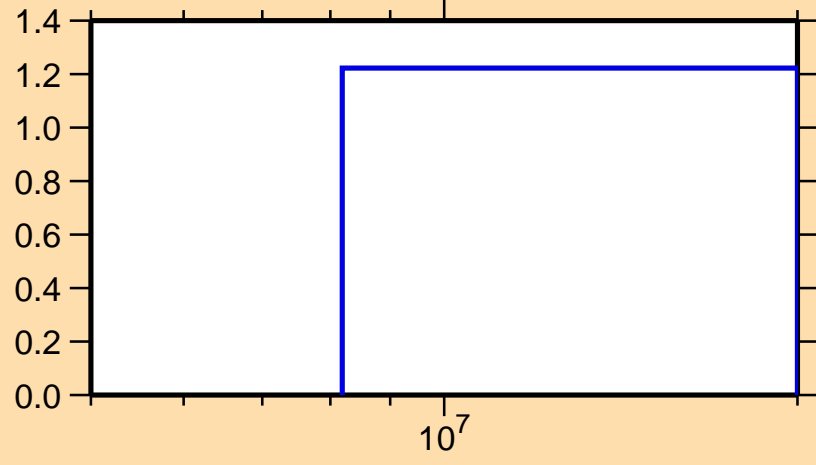
\sigma vs. E for ^{173}\text{Ta}(n,2n)
