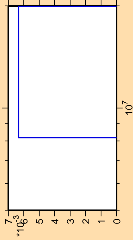
\Delta\sigma/\sigma vs. E for ^{173}\text{Ta}(n,\text{pt})
