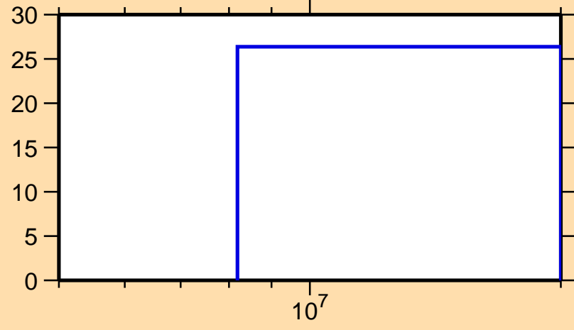
\Delta\sigma/\sigma vs. E for ^{173}\text{Ta}(n,2n)
