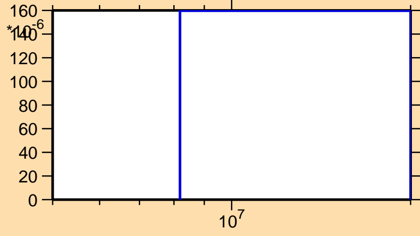
\sigma vs. E for ^{173}\text{Ta}(n,3n)
