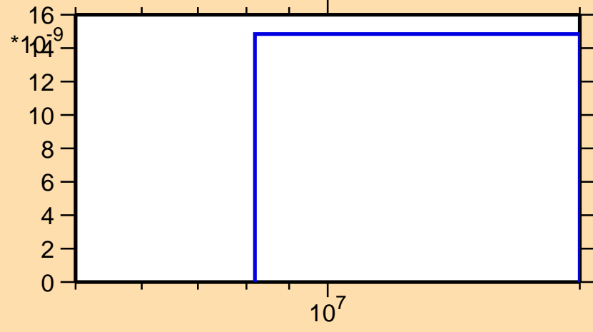
\sigma vs. E for ^{173}\text{Ta}(n,\text{He3})
