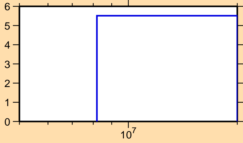
\Delta\sigma/\sigma vs. E for ^{173}\text{Ta}(n,\text{tot.})
