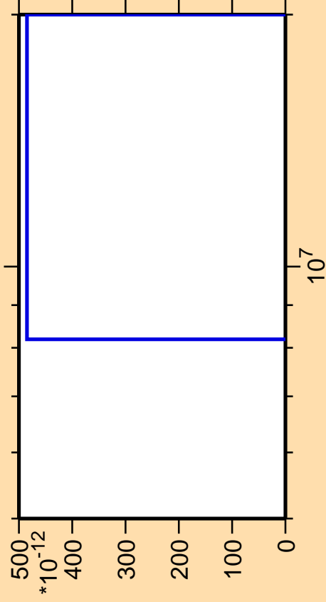
\Delta\sigma/\sigma vs. E for ^{173}\text{Ta} (mt 42)
