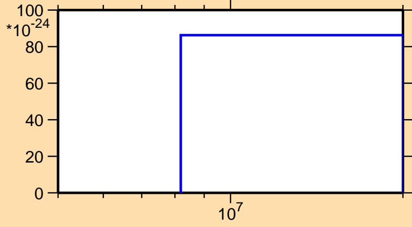
\sigma vs. E for ^{173}\text{Ta} (mt 42)
