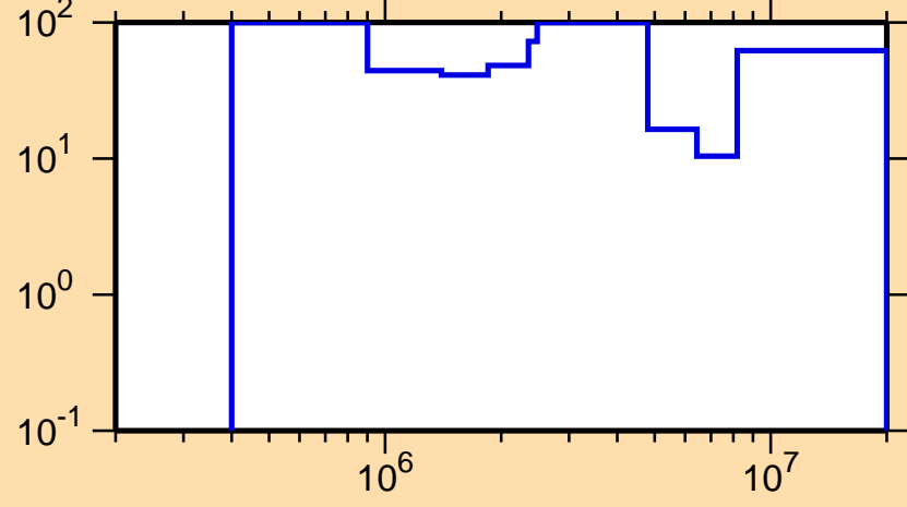
\Delta\sigma/\sigma vs. E for ^{173}\text{Ta}(n,n\text{cont.})
