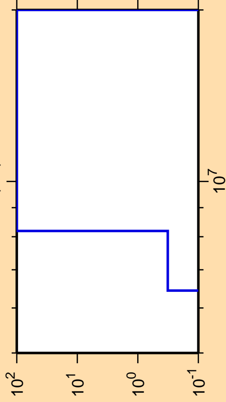
\Delta\sigma/\sigma vs. E for ^{173}\text{Ta}(n,t)
