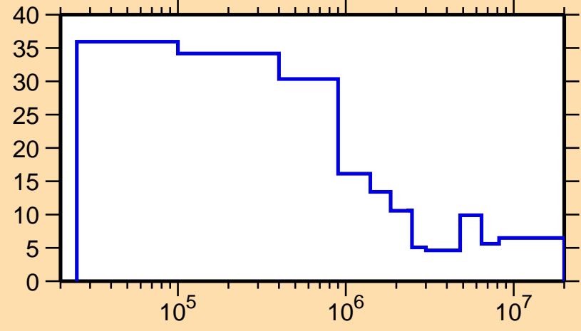
\Delta\sigma/\sigma vs. E for ^{173}\text{Ta}(n,\text{nonel.})
