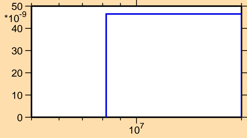
\sigma vs. E for ^{173}\text{Ta}(n,2n\alpha)
