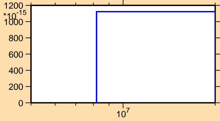
\sigma vs. E for ^{173}\text{Ta}(n,\text{pd})
