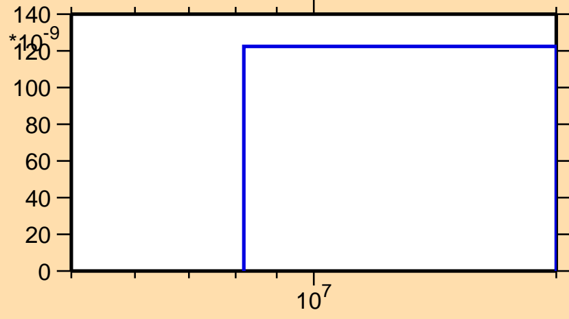
\sigma vs. E for ^{173}\text{Ta}(n,\text{nd})
