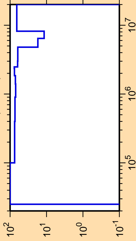
\Delta\sigma/\sigma vs. E for ^{173}\text{Ta}(n,\text{inel.})
