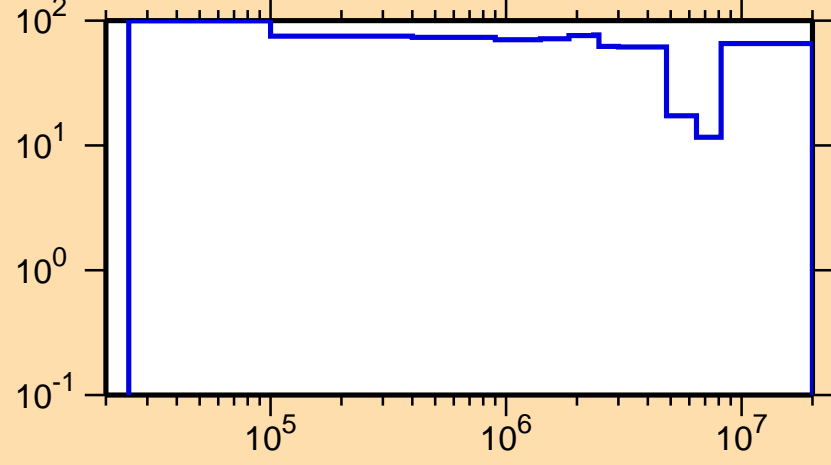
\Delta\sigma/\sigma vs. E for ^{173}\text{Ta}(n,\text{inel.})
