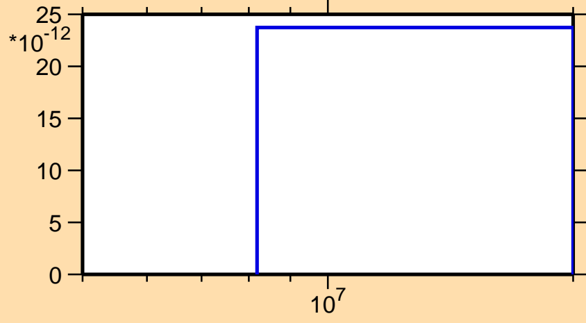
\sigma vs. E for ^{173}\text{Ta}(\text{mt117})
