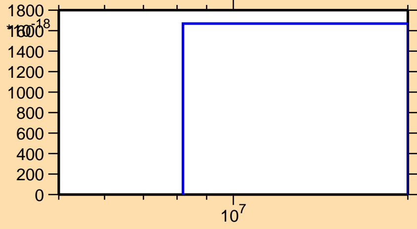
\sigma vs. E for ^{173}\text{Ta}(n,\text{pt})
