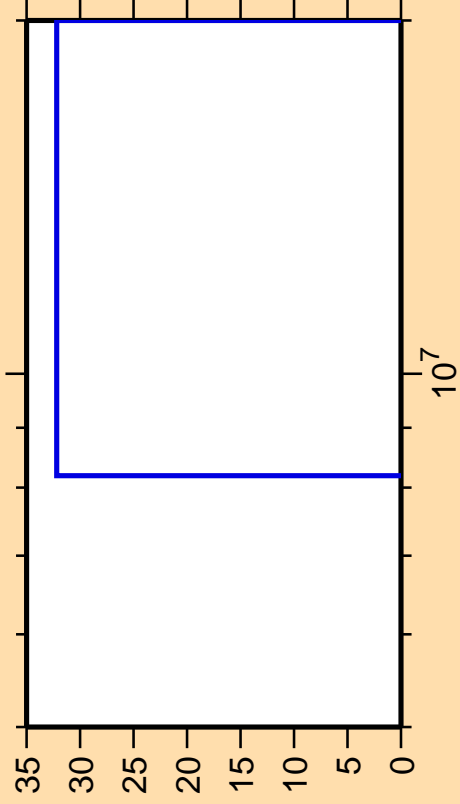
\Delta\sigma/\sigma vs. E for ^{173}\text{Ta}(n,n_1)
