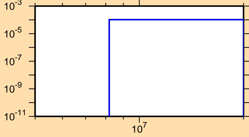
\sigma vs. E for ^{173}\text{Ta}(n,t)
