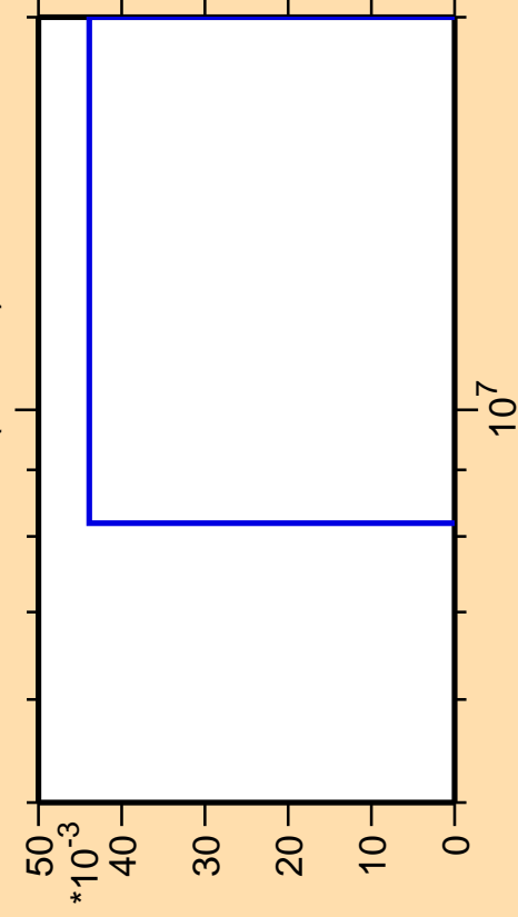
\Delta\sigma/\sigma vs. E for ^{173}\text{Ta} (mt 34)
