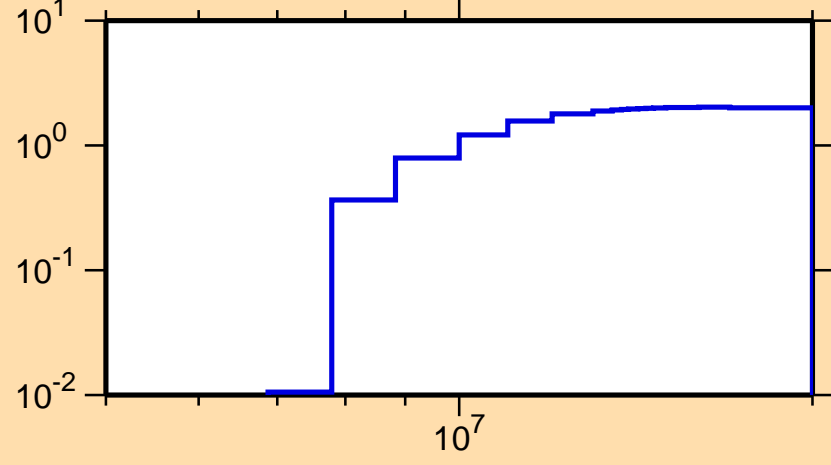
\sigma vs. E for ^{174}\text{Ta}(n,2n)
