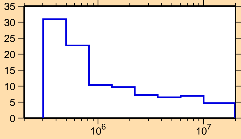
\Delta\sigma/\sigma vs. E for ^{174}\text{Ta}(n,nonel.)
