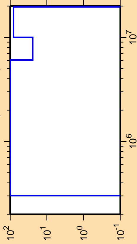
\Delta\sigma/\sigma vs. E for ^{174}\text{Ta}(n,ncont.)
