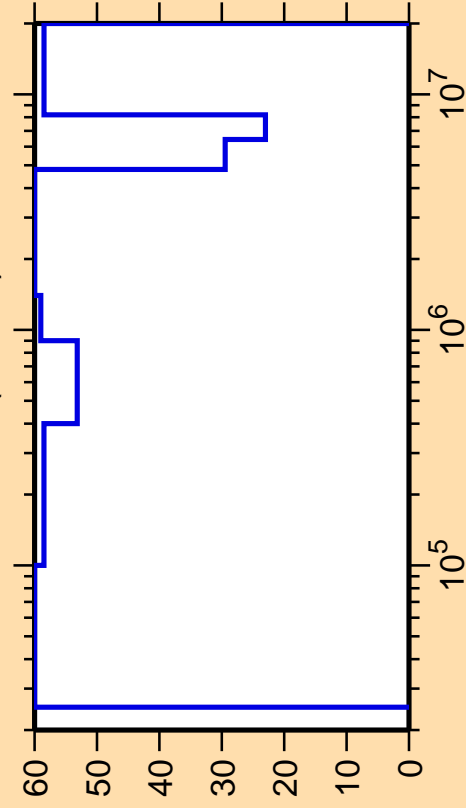
\Delta\sigma/\sigma vs. E for ^{174}\text{Ta}(n,\text{inel.})
