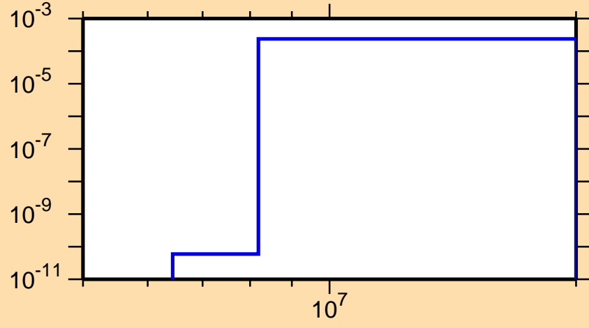
\sigma vs. E for ^{174}\text{Ta}(n,t)
