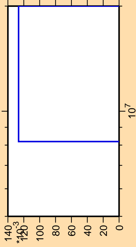
\Delta\sigma/\sigma vs. E for ^{174}\text{Ta}(n,\text{pt})
