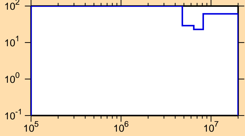
\Delta\sigma/\sigma vs. E for ^{174}\text{Ta}(n,n\text{cont.})
