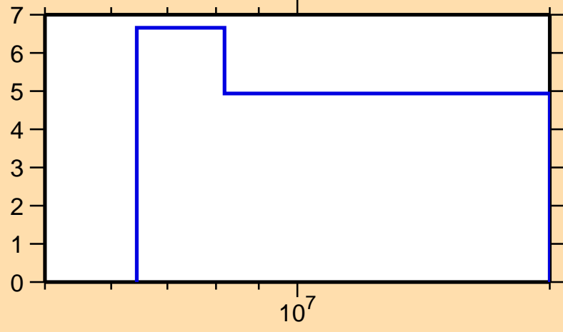
\Delta\sigma/\sigma vs. E for ^{174}\text{Ta}(n,\text{nonel.})
