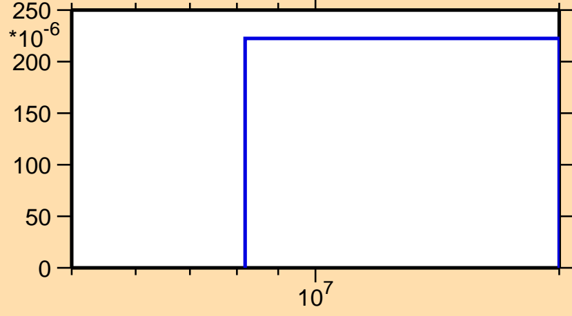
\sigma vs. E for ^{174}\text{Ta}(n,3n)
