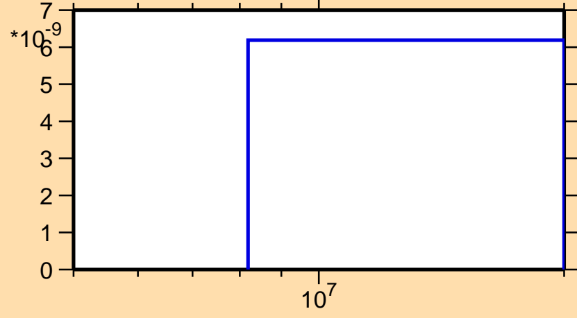
\sigma vs. E for ^{174}\text{Ta}(n,nt)
