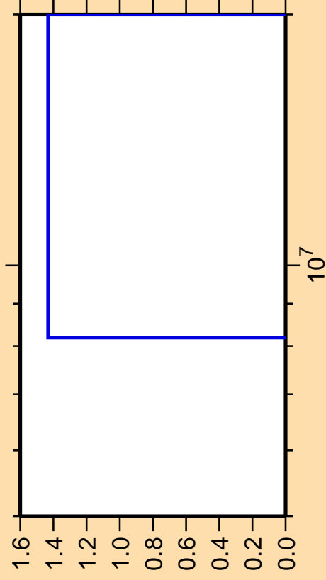
\Delta\sigma/\sigma vs. E for ^{174}\text{Ta} (mt 34)
