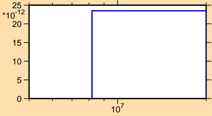
\sigma vs. E for ^{174}\text{Ta}(\text{mt } 45)
