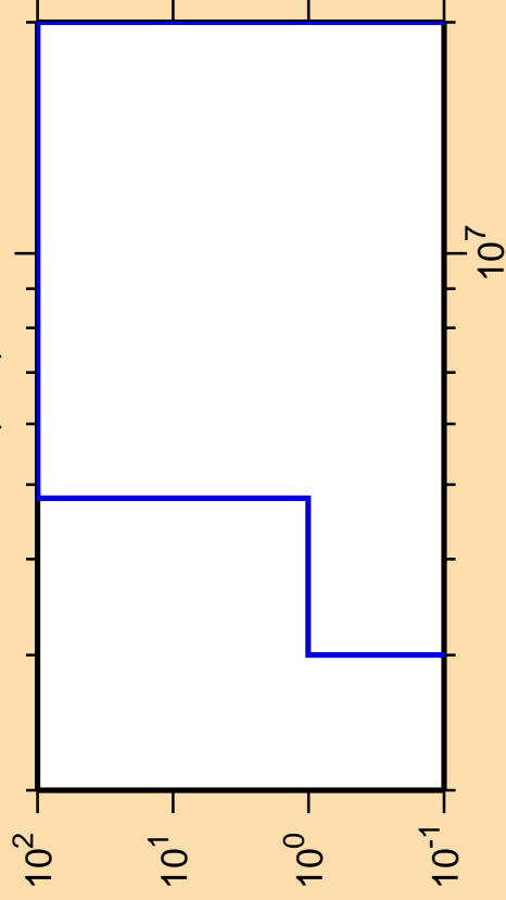
\Delta\sigma/\sigma vs. E for ^{174}\text{Ta}(n,d)
