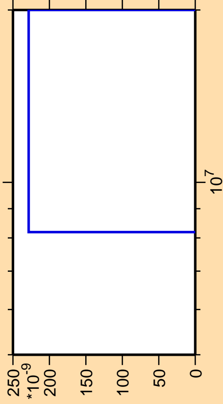
\Delta\sigma/\sigma vs. E for ^{174}\text{Ta} (mt 42)
