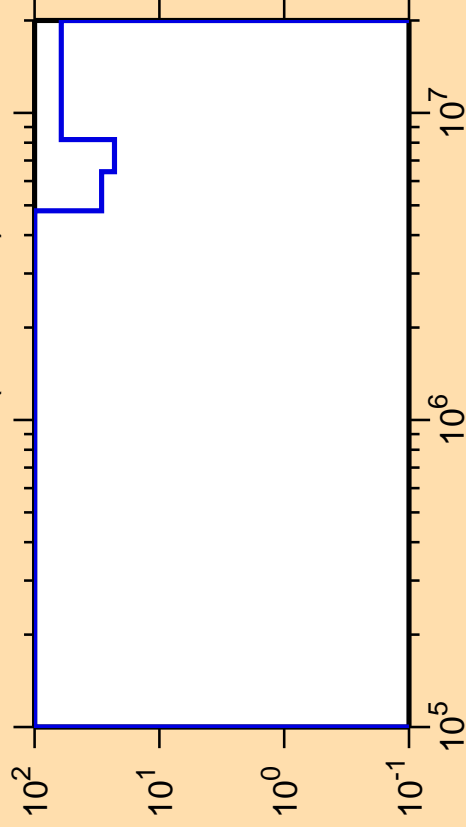
\Delta\sigma/\sigma vs. E for ^{174}\text{Ta}(n,\text{ncont.})
