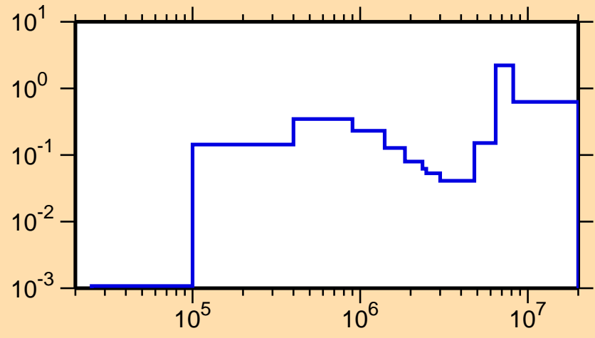
\sigma vs. E for ^{174}\text{Ta}(n,\text{inel.})
