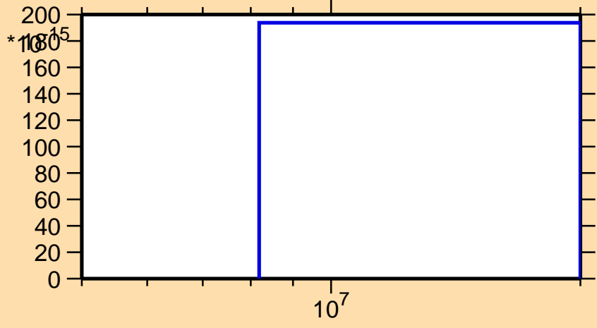
\sigma vs. E for ^{174}\text{Ta} (mt 34)
