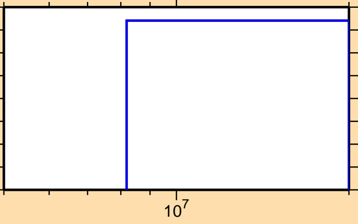
\sigma vs. E for ^{174}\text{Ta}(n,2np)
