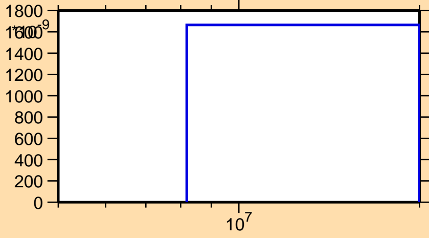
\sigma vs. E for ^{174}\text{Ta}(n,\text{nd})
