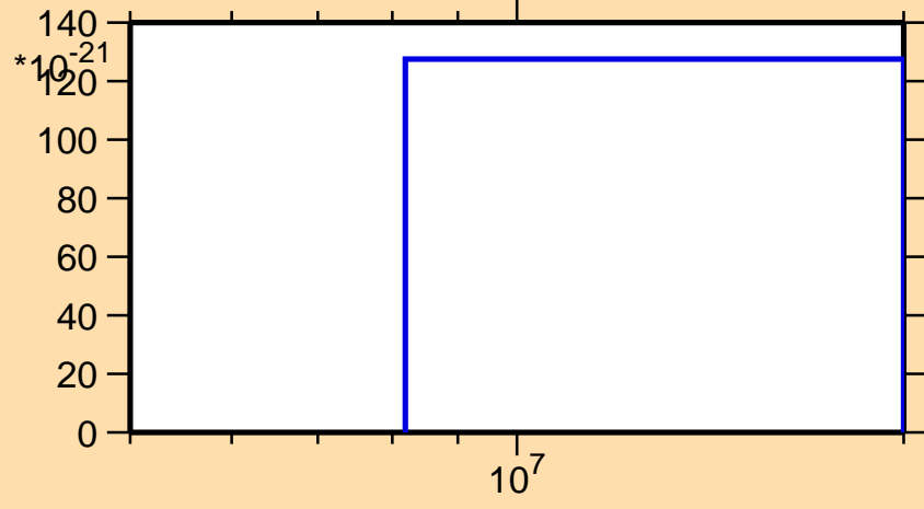
\sigma vs. E for ^{174}\text{Ta} (mt 42)
