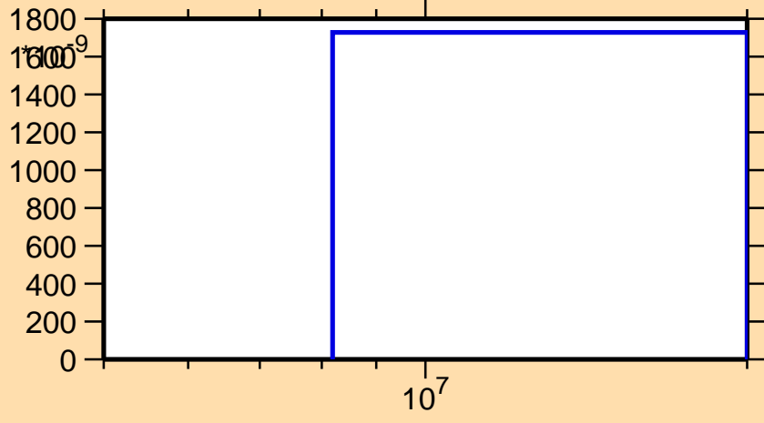
\sigma vs. E for ^{174}\text{Ta}(n,2n\alpha)
