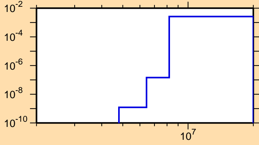
\sigma vs. E for ^{174}\text{Ta}(n,d)
