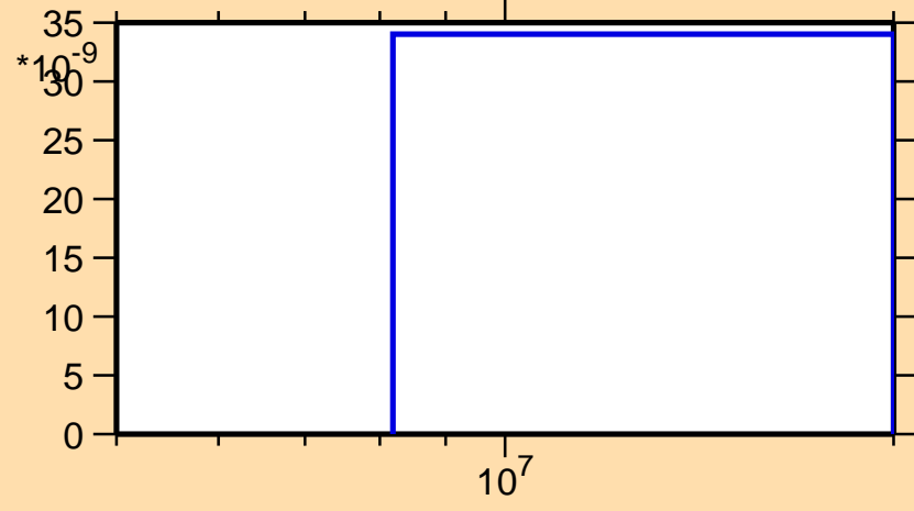
\sigma vs. E for ^{174}\text{Ta}(n,\text{He3})
