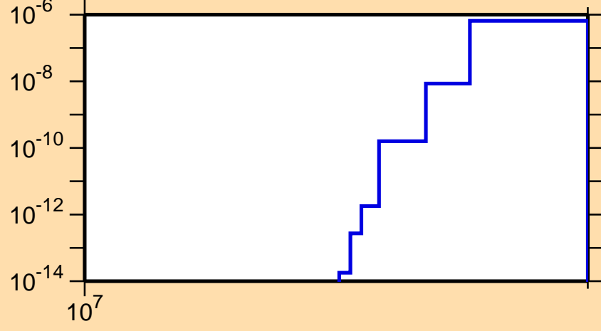
\sigma vs. E for ^{175}\text{Ta}(n,nt)
