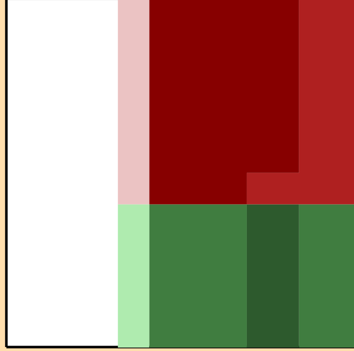
\Delta\sigma/\sigma vs. E for ^{175}\text{Ta}(n,2n)
