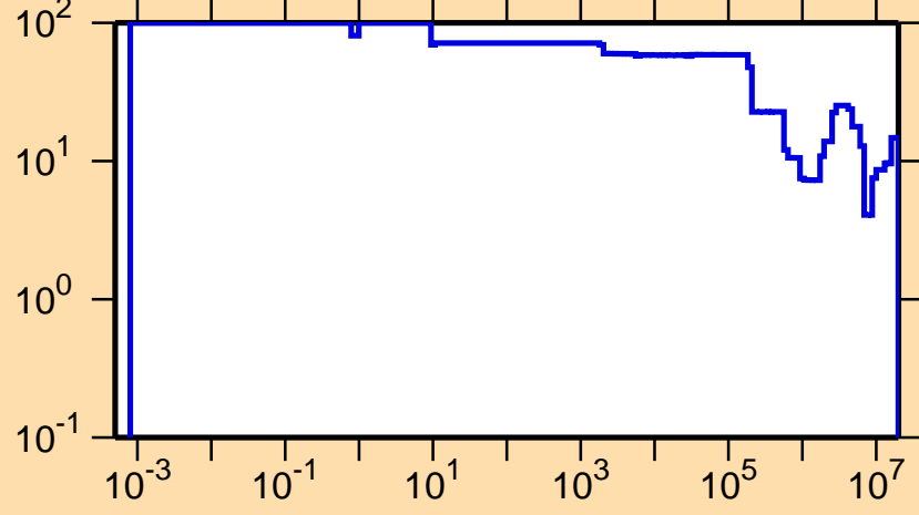
\Delta\sigma/\sigma vs. E for ^{175}\text{Ta}(n,\text{el.})
