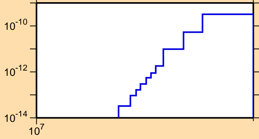
\sigma vs. E for ^{175}\text{Ta}(\text{mt } 45)
