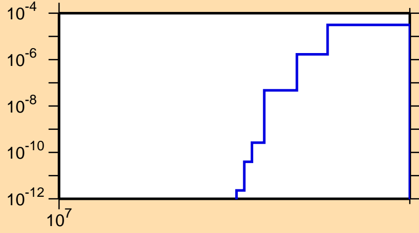
\sigma vs. E for ^{175}\text{Ta}(n,2np)
