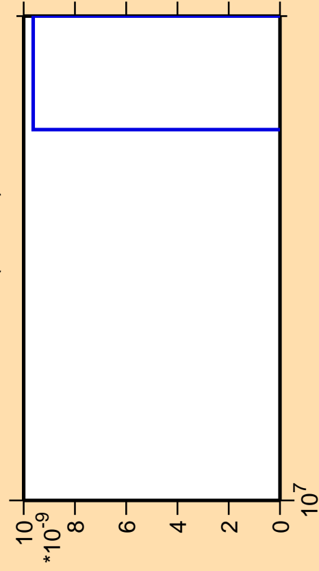
\Delta\sigma/\sigma vs. E for ^{175}\text{Ta} (mt 42)
