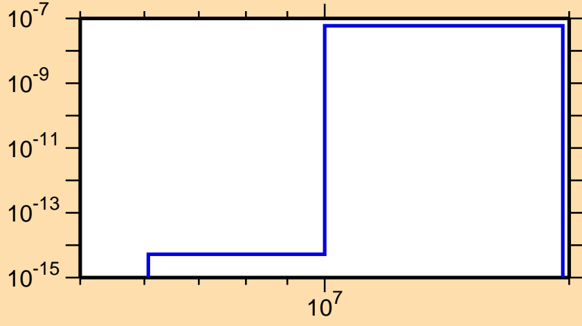
\sigma vs. E for ^{175}\text{Ta}(n,2n\alpha)
