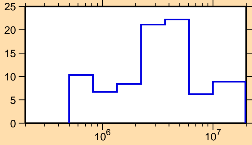
\Delta\sigma/\sigma vs. E for ^{175}\text{Ta}(n,el.)
