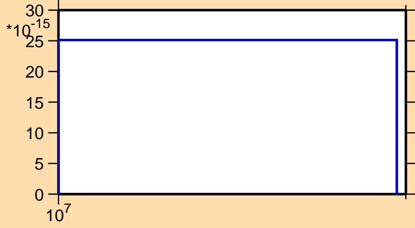
\sigma vs. E for ^{175}\text{Ta}(n,\text{pd})
