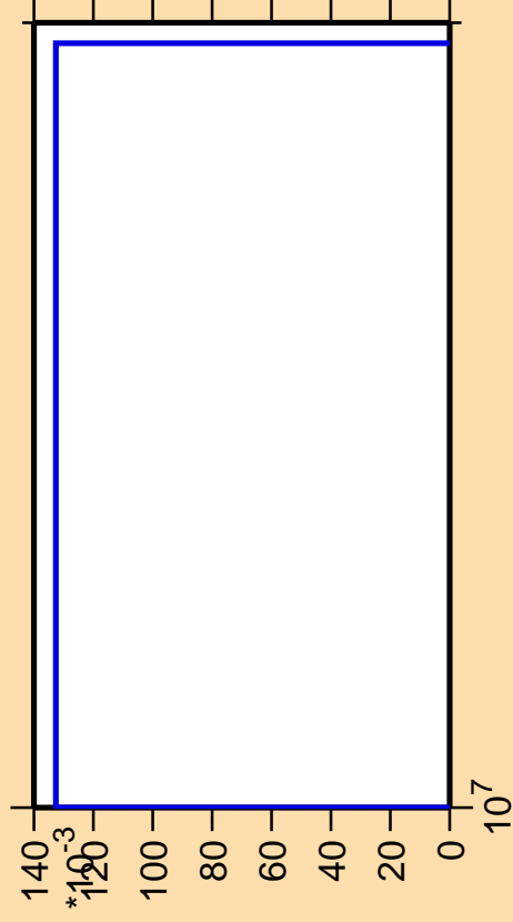
\Delta\sigma/\sigma vs. E for ^{175}\text{Ta}(n,\text{pd})
