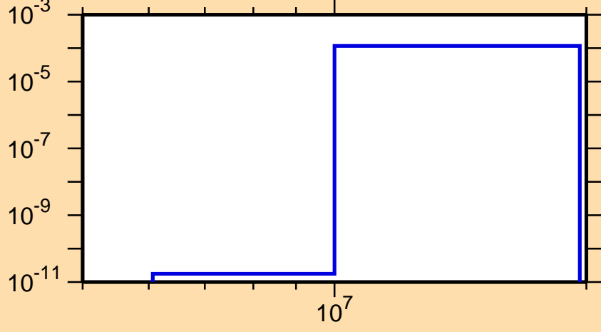
\sigma vs. E for ^{175}\text{Ta}(n,t)
