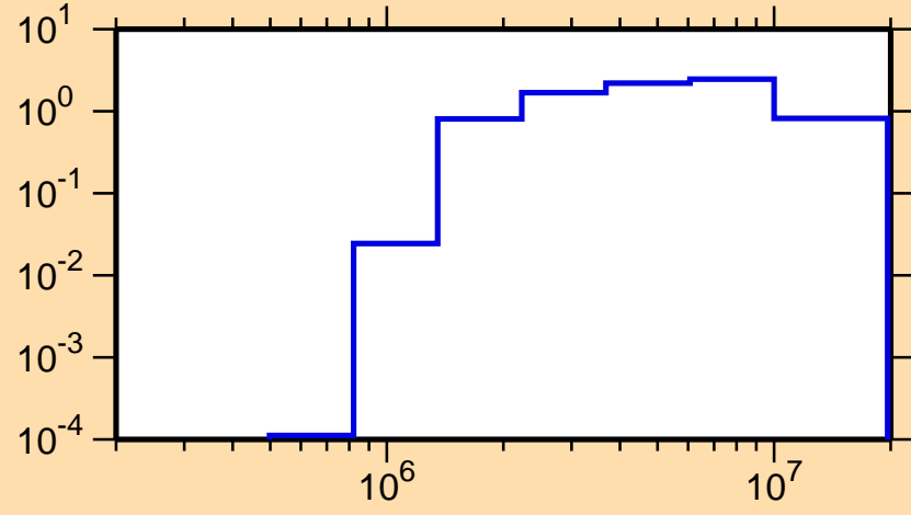
\sigma vs. E for ^{175}\text{Ta}(n,n\text{cont.})
