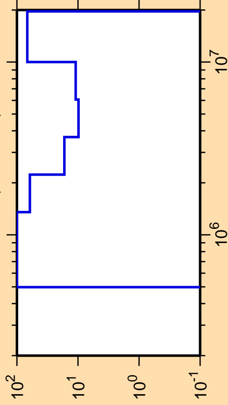
\Delta\sigma/\sigma vs. E for ^{175}\text{Ta}(n,\text{ncont.})
