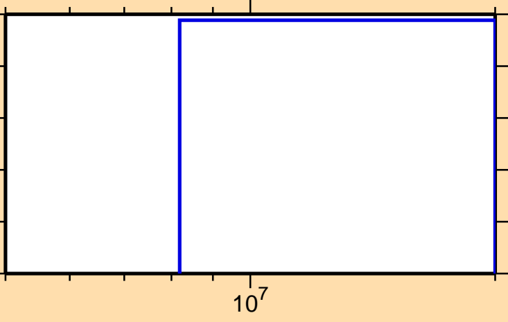
\sigma vs. E for ^{175}\text{Ta}(n,2n\alpha)
