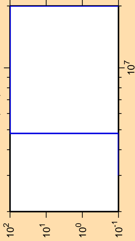
\Delta\sigma/\sigma vs. E for ^{175}\text{Ta}(n,d)
