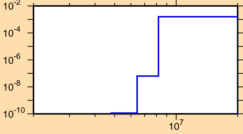
\sigma vs. E for ^{175}\text{Ta}(n,d)
