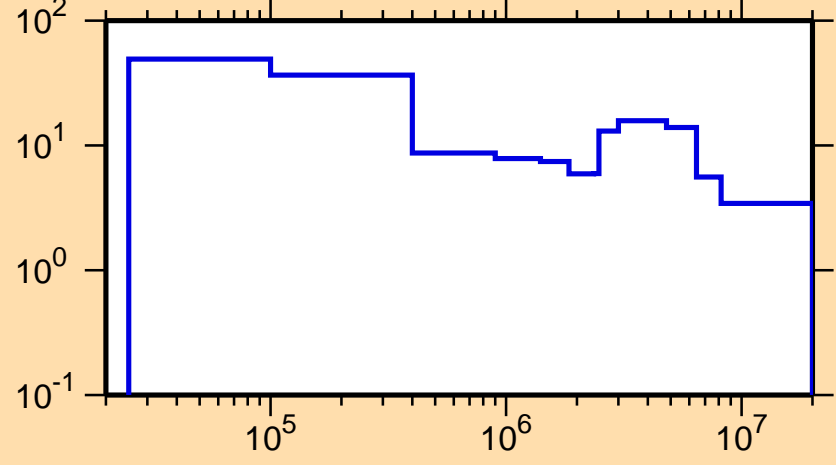
\Delta\sigma/\sigma vs. E for ^{175}\text{Ta}(n,\text{tot.})
