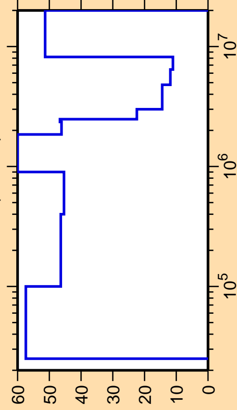
\Delta\sigma/\sigma vs. E for ^{175}\text{Ta}(n,\text{inel.})
