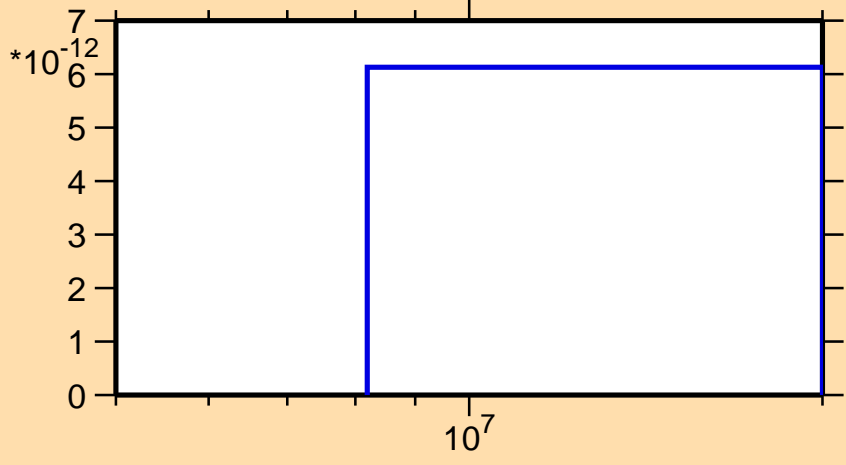
\sigma vs. E for ^{175}\text{Ta}(\text{mt } 45)
