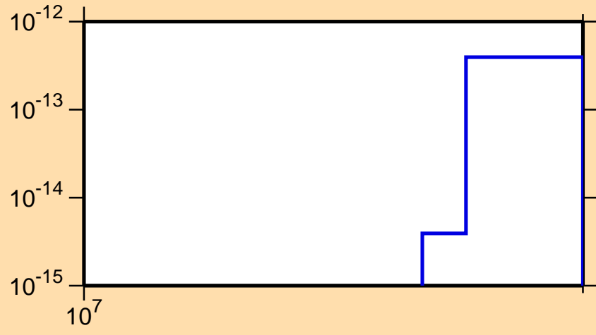
\sigma vs. E for ^{176}\text{Ta}(n,\text{pd})
