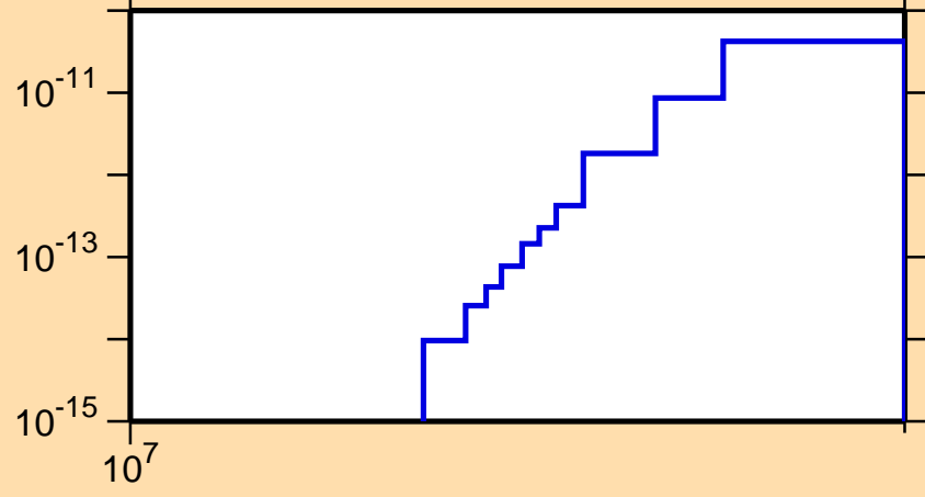
\sigma vs. E for ^{176}\text{Ta}(\text{mt117})
