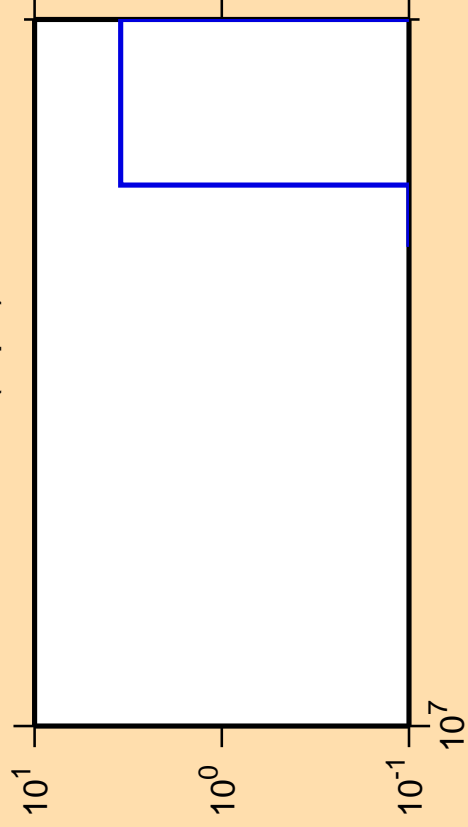
\Delta\sigma/\sigma vs. E for ^{176}\text{Ta}(n,\text{pd})
