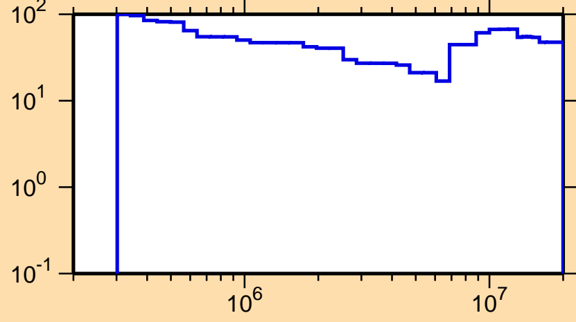
\Delta\sigma/\sigma vs. E for ^{176}\text{Ta}(n,n\text{cont.})
