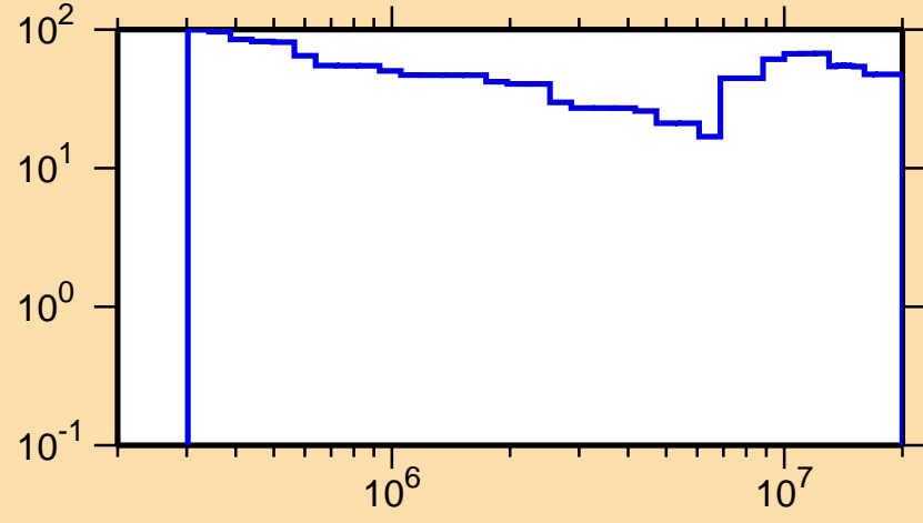
\Delta\sigma/\sigma vs. E for ^{176}\text{Ta}(n,n\text{cont.})
