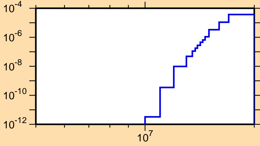
\sigma vs. E for ^{176}\text{Ta}(n,2n\alpha)
