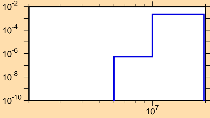
\sigma vs. E for ^{176}\text{Ta}(n,d)
