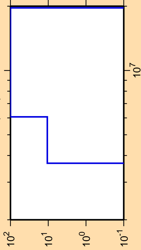
\Delta\sigma/\sigma vs. E for ^{176}\text{Ta}(n,d)
