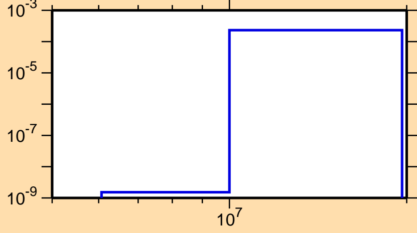
\sigma vs. E for ^{176}\text{Ta}(n,t)
