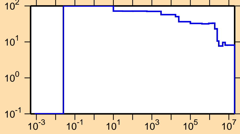
\Delta\sigma/\sigma vs. E for ^{176}\text{Ta}(n,\text{nonel.})
