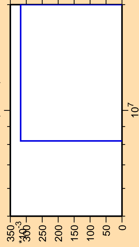
\Delta\sigma/\sigma vs. E for ^{176}\text{Ta}(\text{mt } 34)
