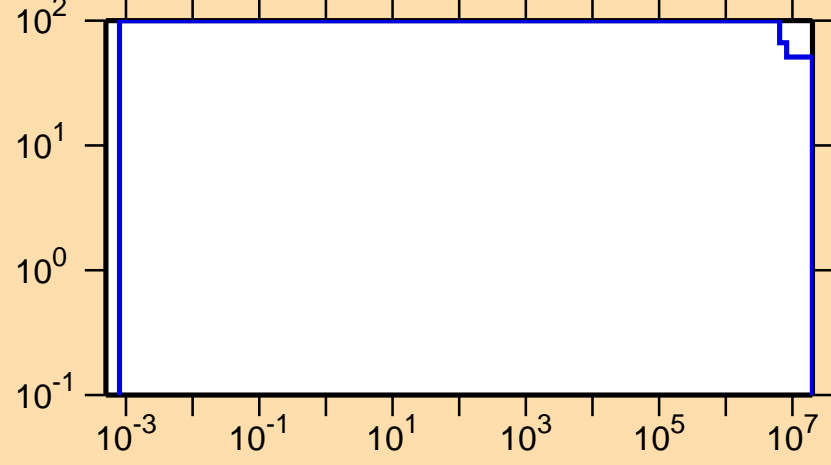
\Delta\sigma/\sigma vs. E for ^{176}\text{Ta}(n,p)
