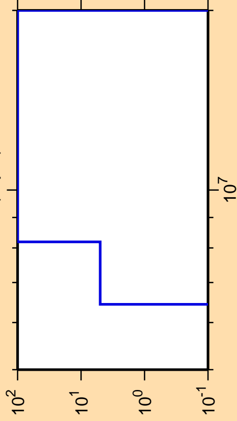
\Delta\sigma/\sigma vs. E for ^{176}\text{Ta}(n,p\alpha)
