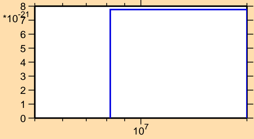
\sigma vs. E for ^{176}\text{Ta}(\text{mt } 42)
