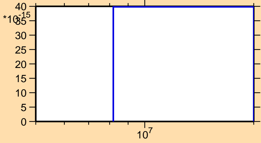
\sigma vs. E for ^{176}\text{Ta}(\text{mt } 34)
