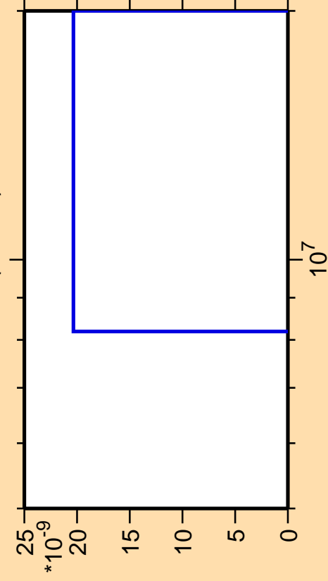
\Delta\sigma/\sigma vs. E for ^{176}\text{Ta}(\text{mt } 42)
