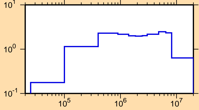
\sigma vs. E for ^{176}\text{Ta}(n,\text{inel.})
