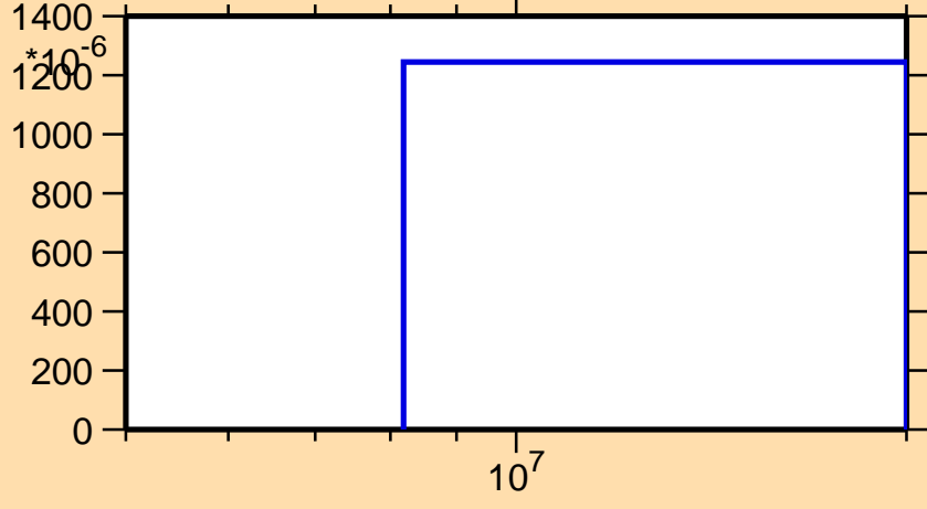
\sigma vs. E for ^{176}\text{Ta}(n,3n)
