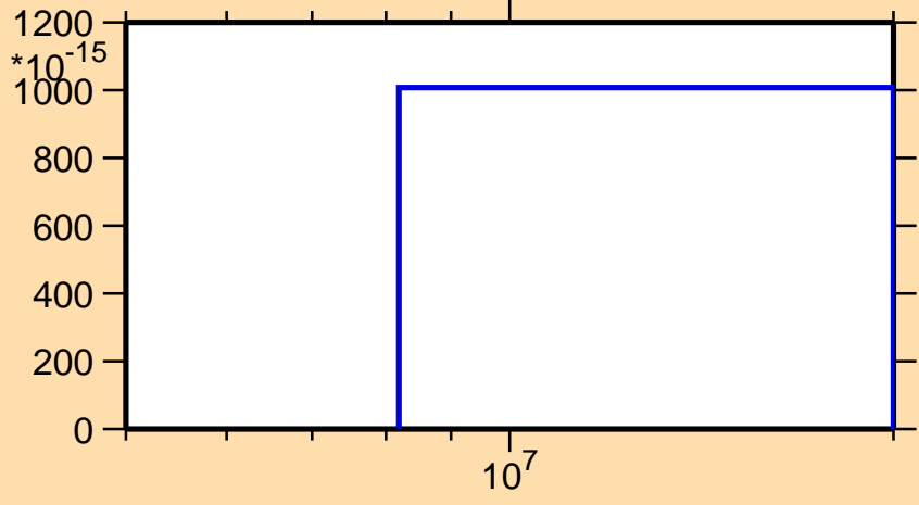
\sigma vs. E for ^{176}\text{Ta}(\text{mt } 45)
