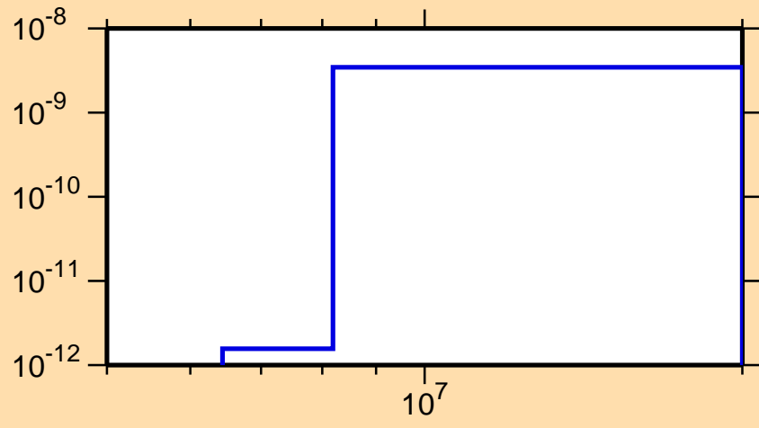
\sigma vs. E for ^{176}\text{Ta}(n,p\alpha)
