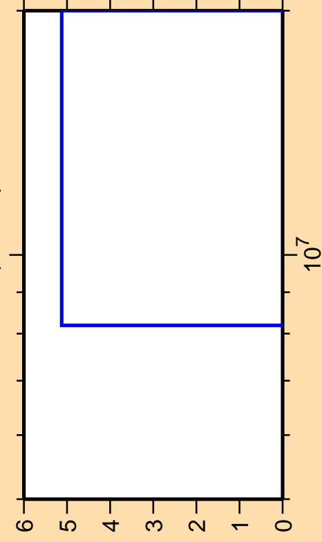
\Delta\sigma/\sigma vs. E for ^{176}\text{Ta}(\text{mt } 45)
