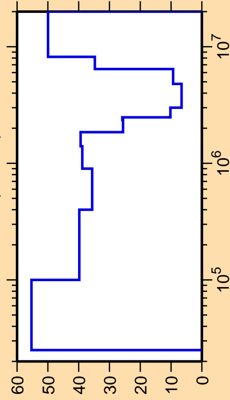
\Delta\sigma/\sigma vs. E for ^{176}\text{Ta}(n,\text{inel.})
