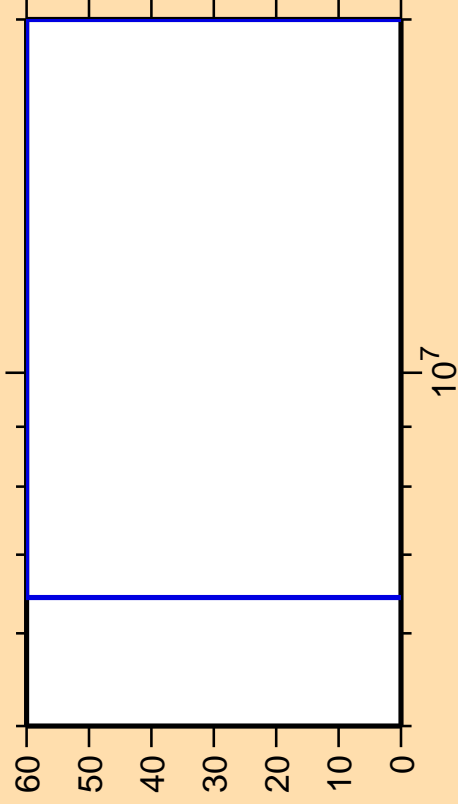
\Delta\sigma/\sigma vs. E for ^{176}\text{Ta}(n,\gamma)
