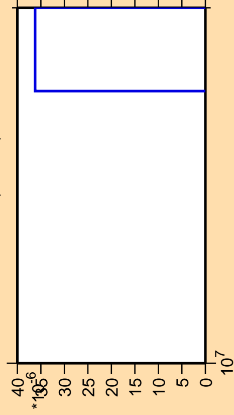
\Delta\sigma/\sigma vs. E for ^{177}\text{Ta} (mt 42)
