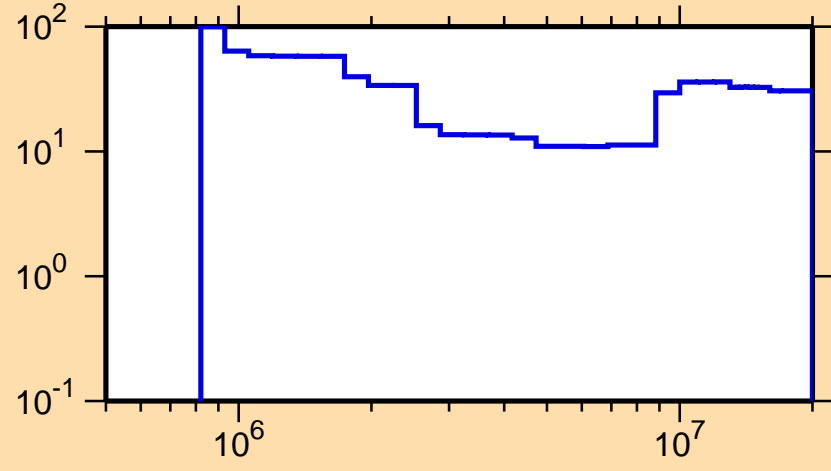
\Delta\sigma/\sigma vs. E for ^{177}\text{Ta}(n,ncont.)
