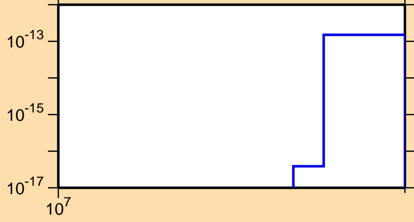
\sigma vs. E for ^{177}\text{Ta}(n,3n\alpha)
