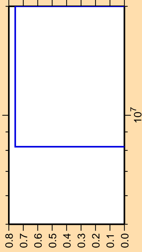
\Delta\sigma/\sigma vs. E for ^{177}\text{Ta}(\text{mt } 45)
