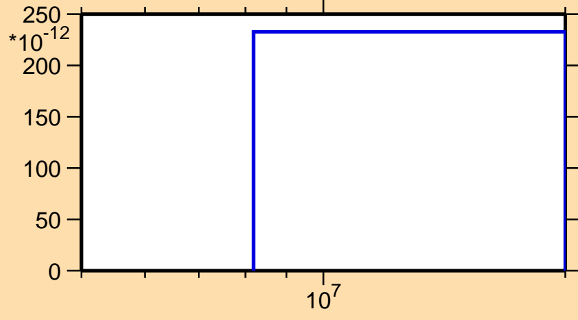
\sigma vs. E for ^{177}\text{Ta}(n,p\alpha)
