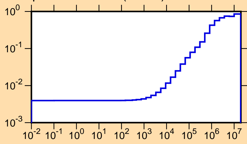
\mu vs. E for ^{178}\text{Ta}(\text{mt251})
