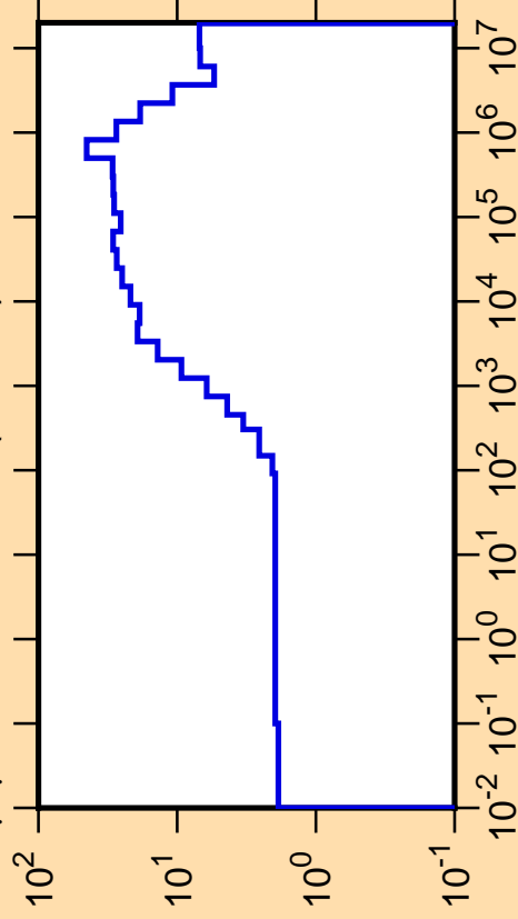
\Delta\mu/\mu vs. E for ^{178}\text{Ta}(\text{mt251})
