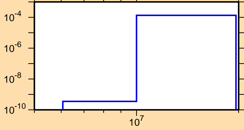
\sigma vs. E for ^{178}\text{Ta}(n,t)
