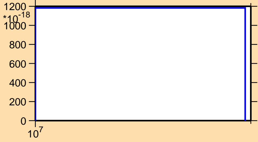
\sigma vs. E for ^{178}\text{Ta} (mt 34)
