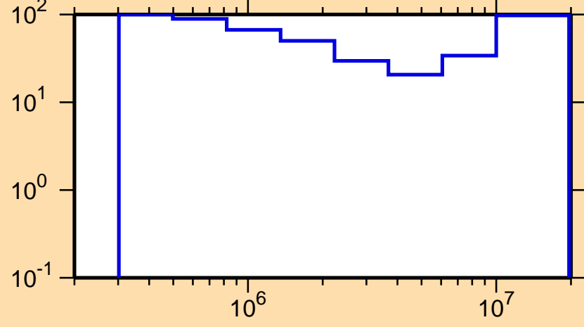
\Delta\sigma/\sigma vs. E for ^{178}\text{Ta}(n,ncont.)
