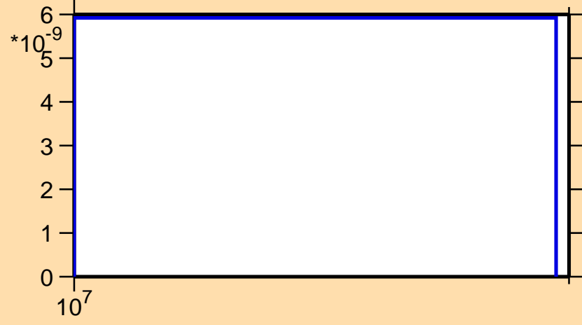
\sigma vs. E for ^{178}\text{Ta}(n,nt)
