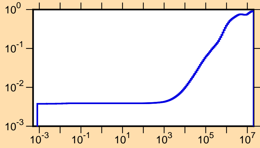
\mu vs. E for ^{179}\text{Ta}(\text{mt251})
