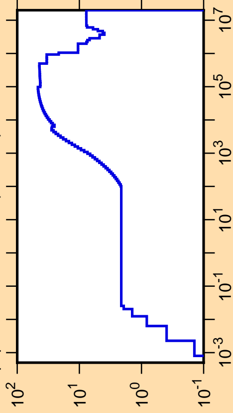
\Delta\mu/\mu vs. E for ^{179}\text{Ta}(\text{mt251})
