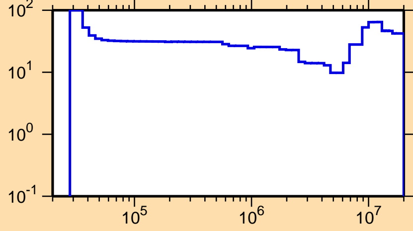
\Delta\sigma/\sigma vs. E for ^{179}\text{Ta}(n,\text{inel.})
