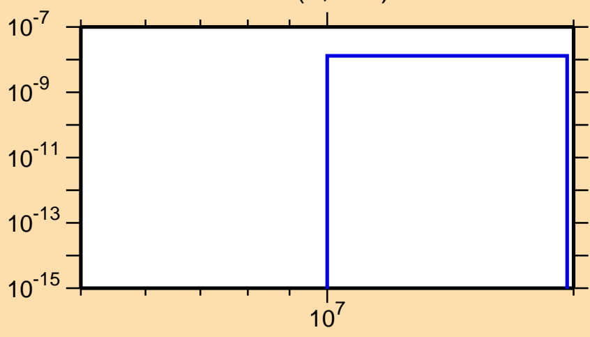
\sigma vs. E for ^{179}\text{Ta}(n,2n\alpha)
