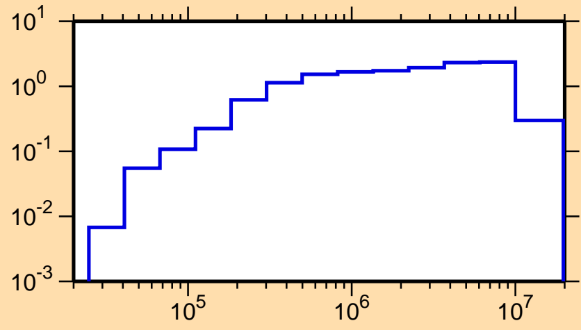
\sigma vs. E for ^{179}\text{Ta}(n,\text{inel.})
