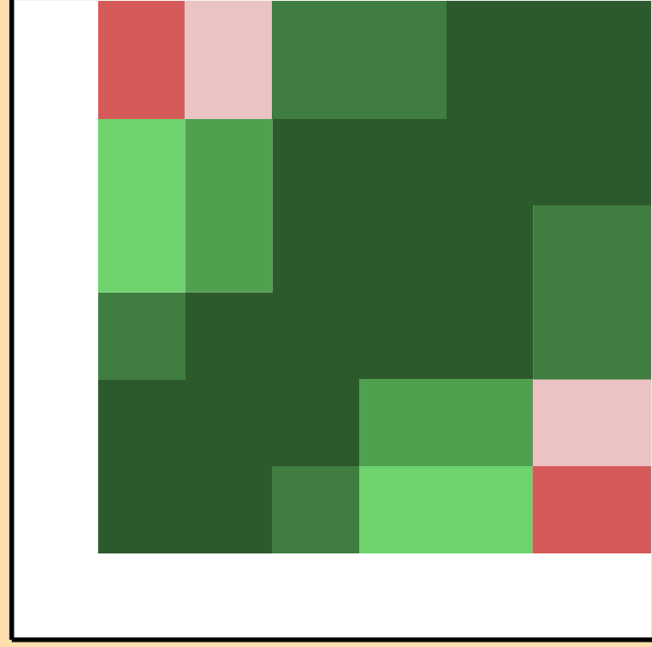
\sigma vs. E for ^{179}\text{Ta}(n,n\text{cont.})
