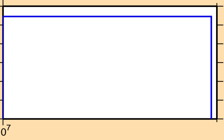
\sigma vs. E for ^{179}\text{Ta}(n,3n)
