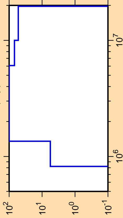
\Delta\sigma/\sigma vs. E for ^{179}\text{Ta}(n,p)
