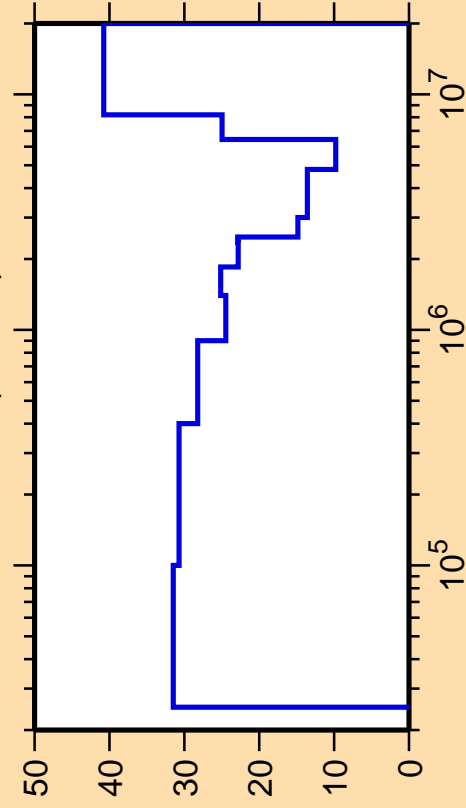
\Delta\sigma/\sigma vs. E for ^{179}\text{Ta}(n,\text{inel.})
