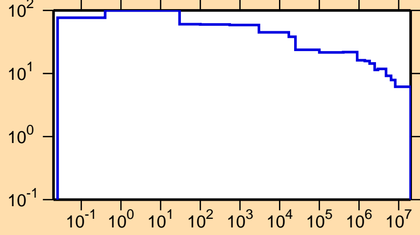
\Delta\sigma/\sigma vs. E for ^{179}\text{Ta}(n,\text{nonel.})
