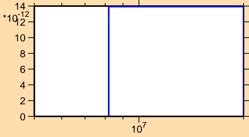
\sigma vs. E for ^{179}\text{Ta}(n,\text{He}3)
