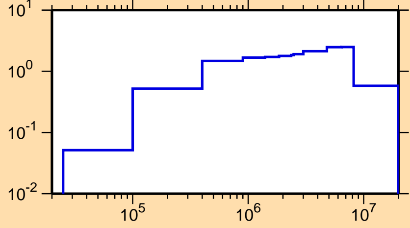
\sigma vs. E for ^{179}\text{Ta}(n,\text{inel.})
