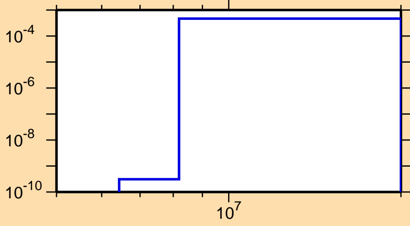
\sigma vs. E for ^{179}\text{Ta}(n,d)
