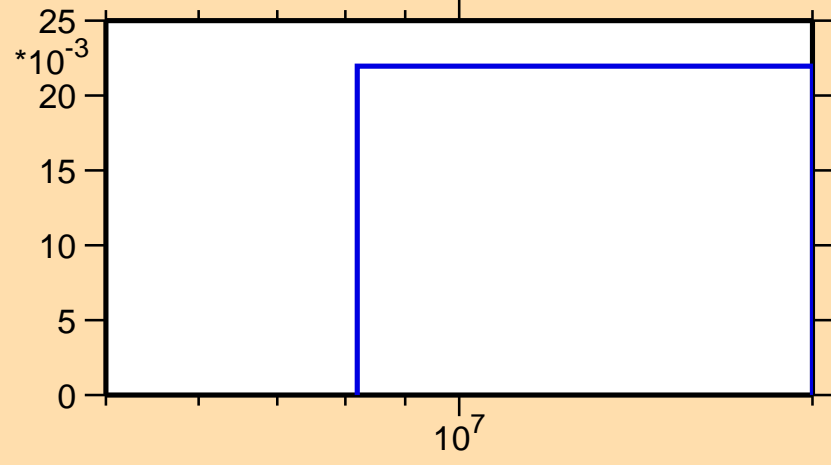
\sigma vs. E for ^{179}\text{Ta}(n,3n)
