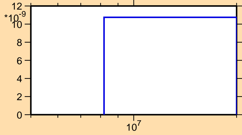
\sigma vs. E for ^{179}\text{Ta}(n,2n\alpha)
