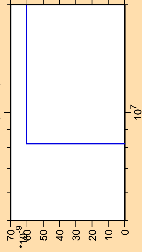
\Delta\sigma/\sigma vs. E for ^{179}\text{Ta} (mt 42)
